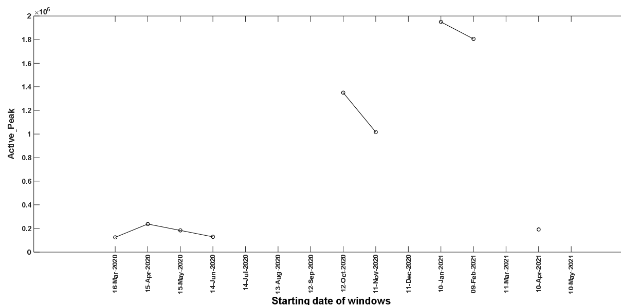
Figure 8. Active_Peak values for windows from 16 th March 2020 till 10 th May 2021 for the UK.
