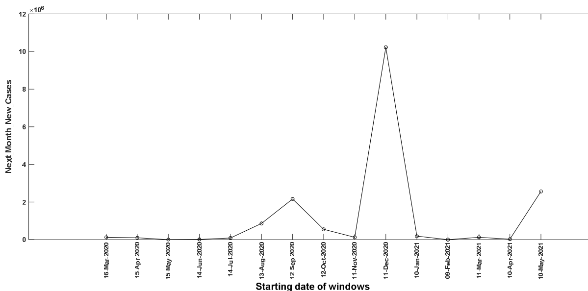
Figure 7. Next_Month_New_Cases values for windows from 16 th March 2020 till 10 th May 2021 for the UK.
