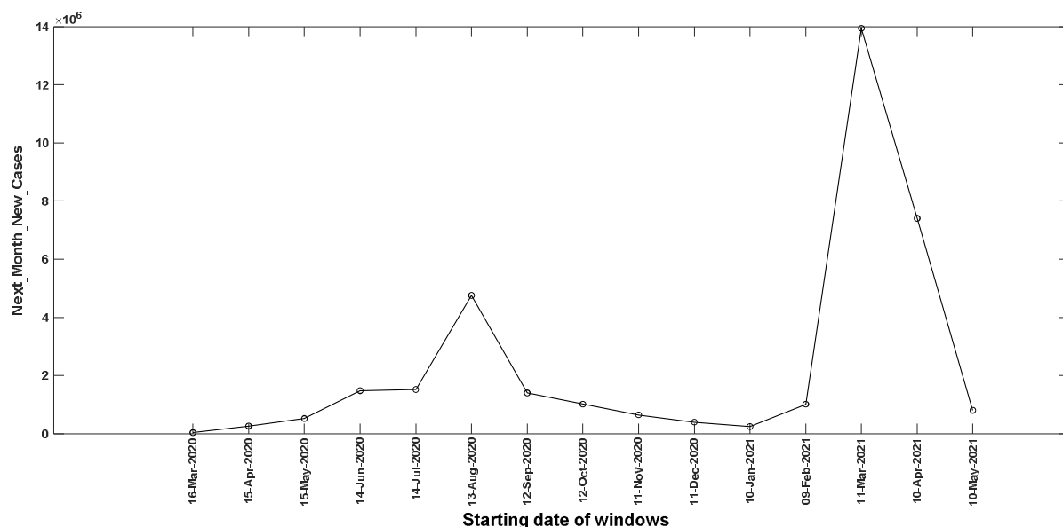
Figure 1. Characteristics of windows starting from 16 th March 2020 till 10 th May 2021 for India.
