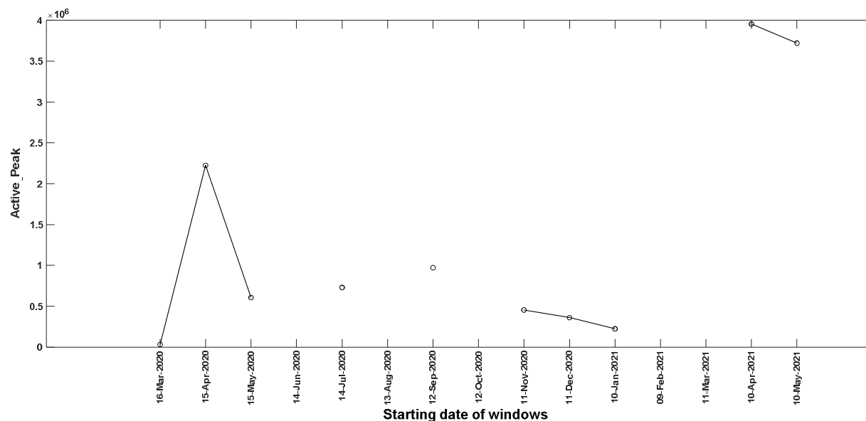
Figure 3. Active_Peak values for windows from 16 th March 2020 till 10 th May 2021 for India.
