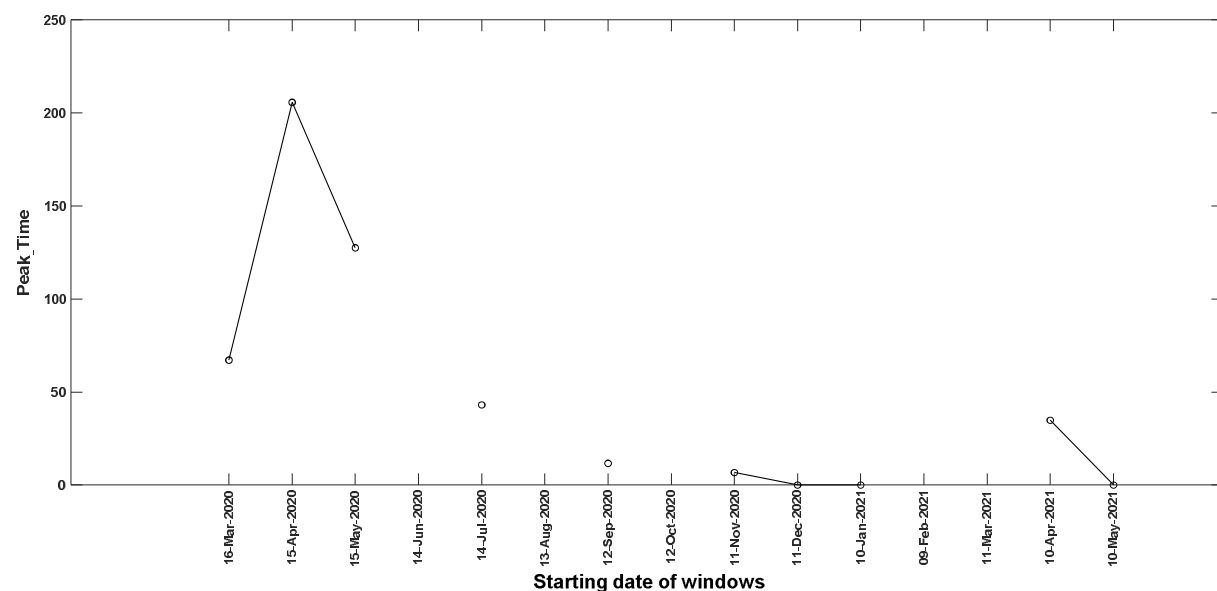
Figure 4. Peak_Time values for windows from 16 th March 2020 till 10 th May 2021 for India.
