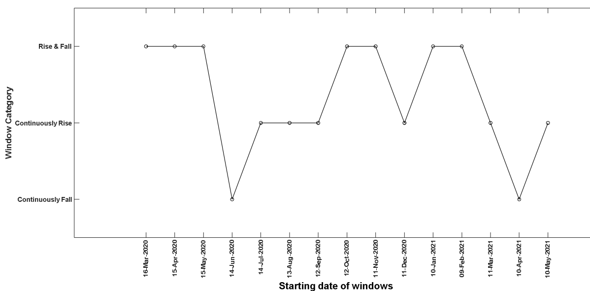
Figure 6. Characteristics of windows starting from 16 th March 2020 till 10 th May 2021 for the UK.
