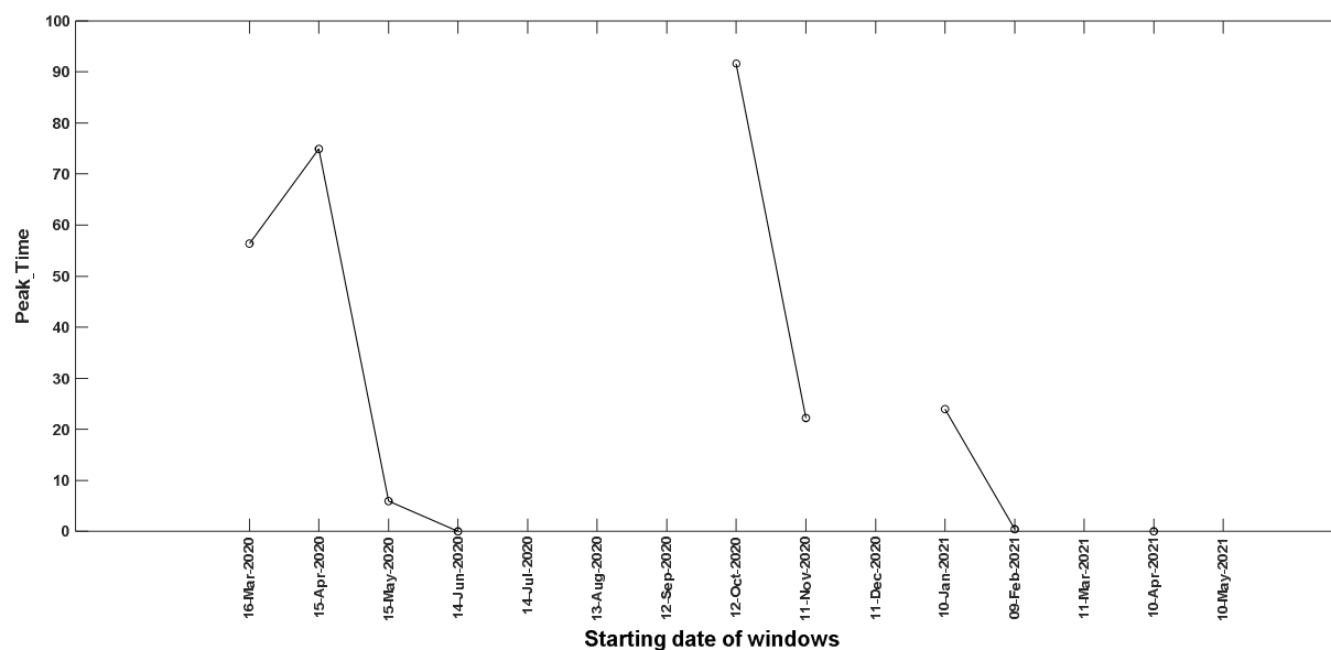
Figure 9. Peak_Time values for windows from 16 th March 2020 till 10 th May 2021 for the UK.
