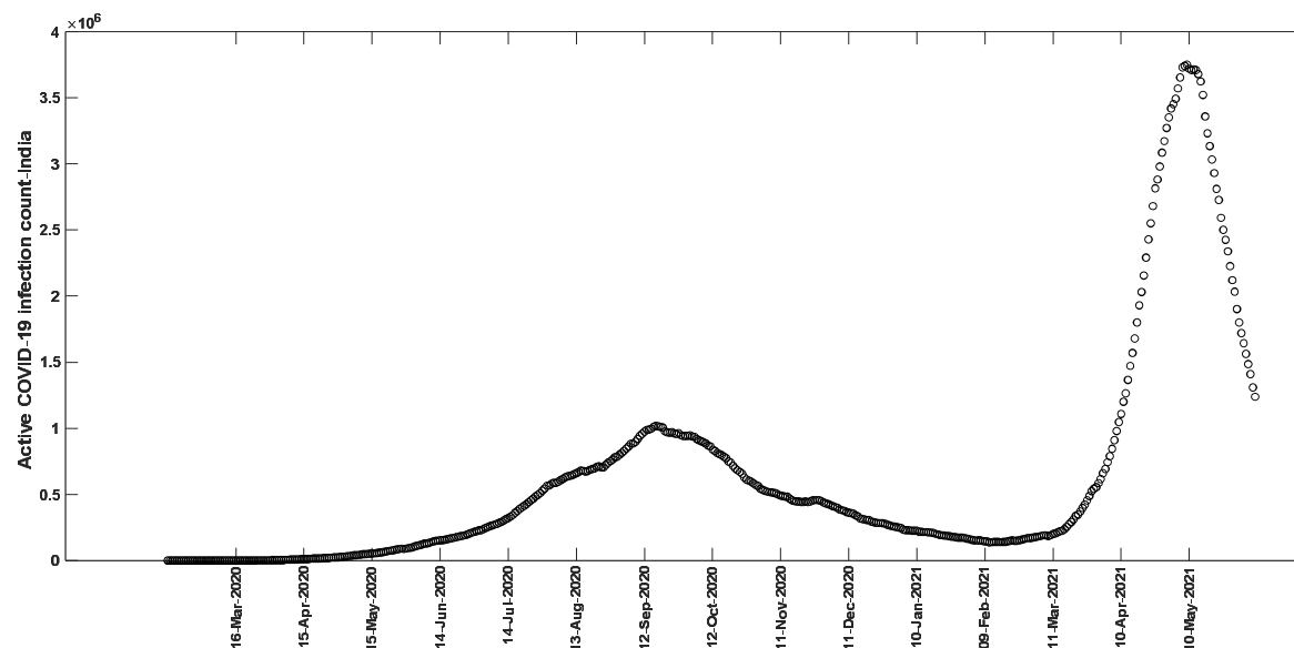
Figure 5. Actual COVID-19 active cases data for India [9].
