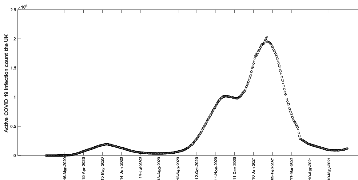
Figure 10. Actual COVID-19 active cases data for the UK [10].
