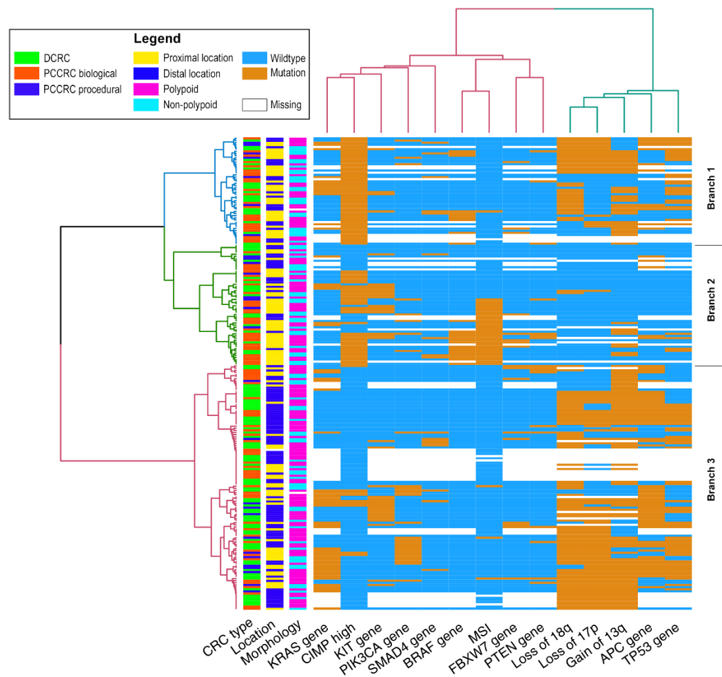
Figure 3: Unsupervised hierarchal cluster analysis based on the molecular features of all CRCs analysed. In the cluster analysis results of the nine genes most commonly mutated in this study (APC, TP53, KRAS, KIT, PIK3CA, BRAF, FBXW7, SMAD4 and PTEN), the significant chromosomal alterations (loss of 17p, loss of 18q and gain of 13q), CIMP status and MSI, were included.
