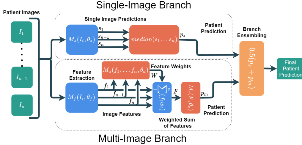
Figure 2: Overview of hybrid machine learning system. The SIL branch processes each image from a patient PBS scan individually. The outputs are then aggregated to produce a single prediction (using the median of the single image predictions). The MIL branch collectively analyzes all of a patient’s images simultaneously, producing one prediction per patient. This is accomplished by first extracting learned per-image features, and then feeding those features into an attention module. The attention module assigns weights (summing to one) to each learned feature. The weights are used to compute a weighted sum across image features, the result of which is passed into a classification module to produce the MIL patient prediction. These two strategies are combined through ensembling, where the outputs of each branch are averaged to produce the final outcome.
