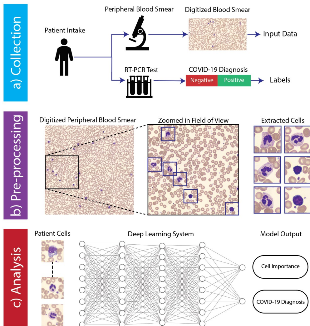
Figure 1: Workflow of automated COVID-19 infection analysis from peripheral blood smear (PBS) image data. a) Data collection procedure at Duke University Medical Center. Subjects randomly selected from patient population subset whom had both a COVID-19 RT-PCR test (ground truth labels) and images from a digital PBS scan (input data). All data was collected anonymously, retaining only the results of the RT-PCR test and digitized PBS images. b) Summary of pre-processing pipeline, where individual images of white blood cells are extracted from the full slide using a high-resolution oil-immersion microscope. c) Data analysis strategy. All cells from a patient are collectively analyzed by a deep neural network to produce both a COVID-19 diagnosis and per-cell importance score.
