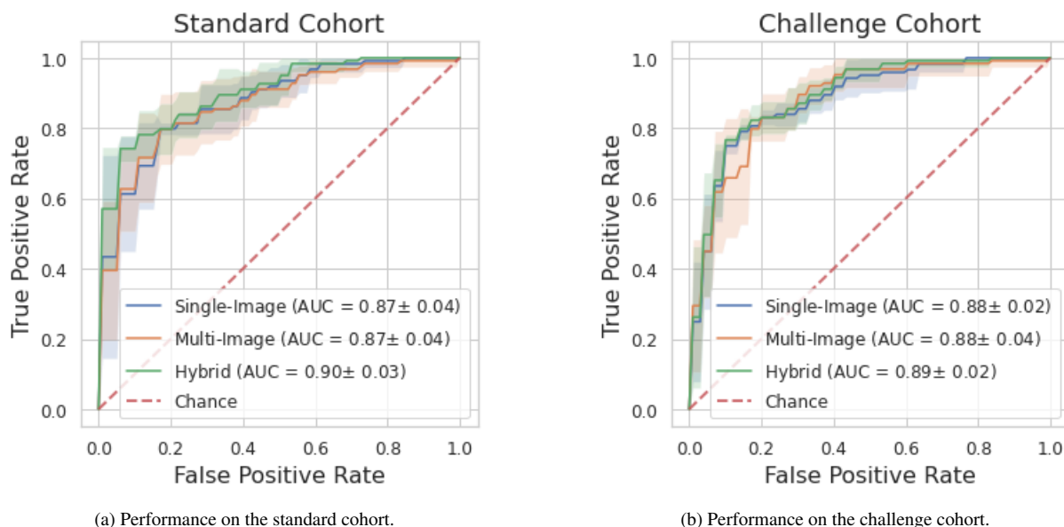
Figure 3: Performance of COVID-19 diagnosis from blood cell morphology analysis as measured by the receiver operator characteristic (ROC). Classification accuracy was 79% and 82% for the standard and challenge cohorts respectively. a) Results reported are the average across the entire dataset, k-fold cross validation was used to maintain independence between the training and test sets. b) COVID-19 positive patients were randomly selected from the standard cohort to counterbalance the COVID-19 negative patients from the challenge cohort (ROC-AUC calculation requires both positive and negative examples).
