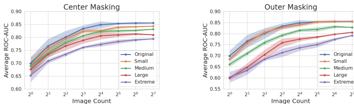
Figure 6: Results of perturbation experiments. Average ROC-AUC of screening predictions compared to number of images (randomly selected across five trials) used to make the prediction.
