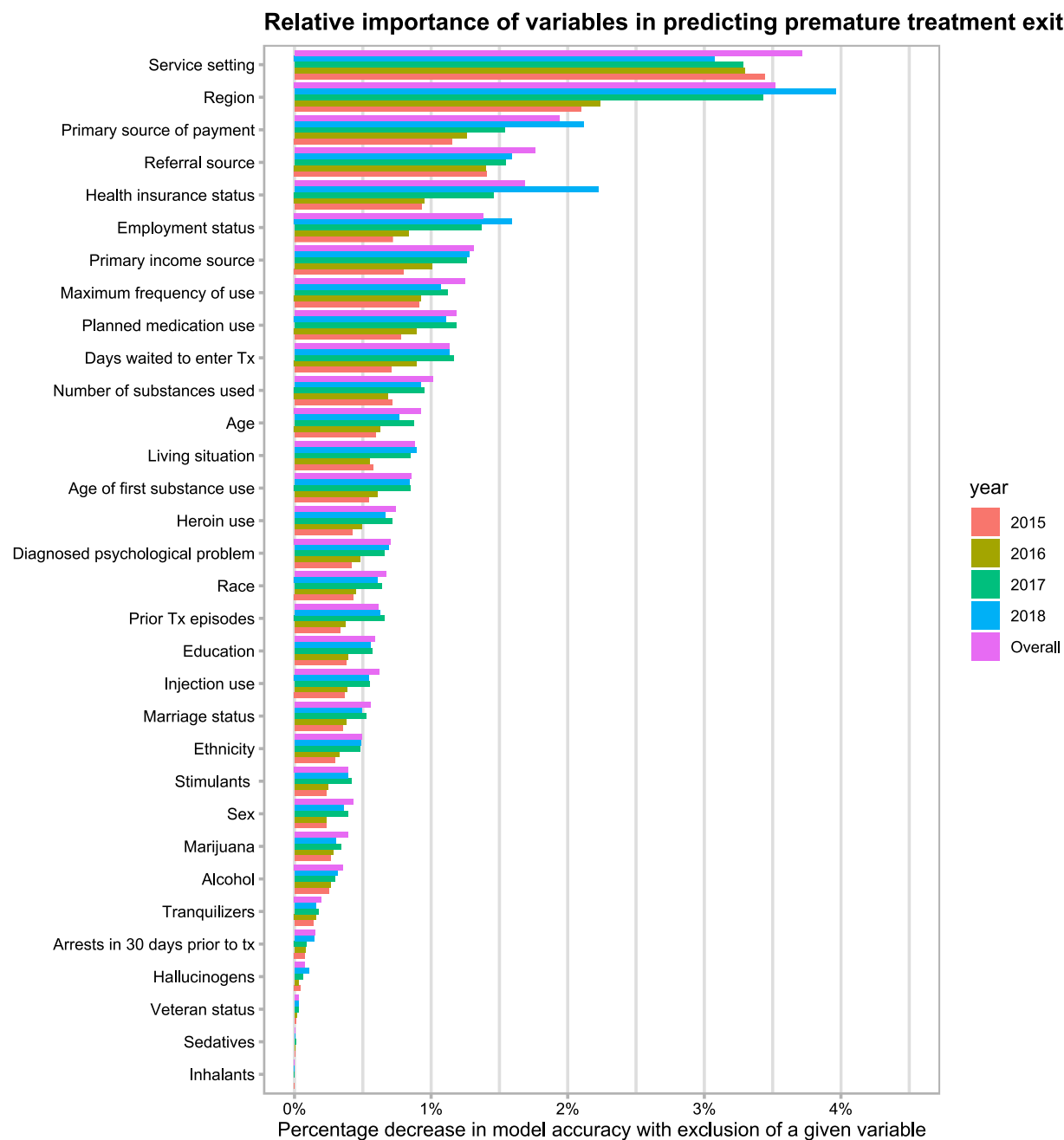
Figure S2. Variable importance stratified by year
