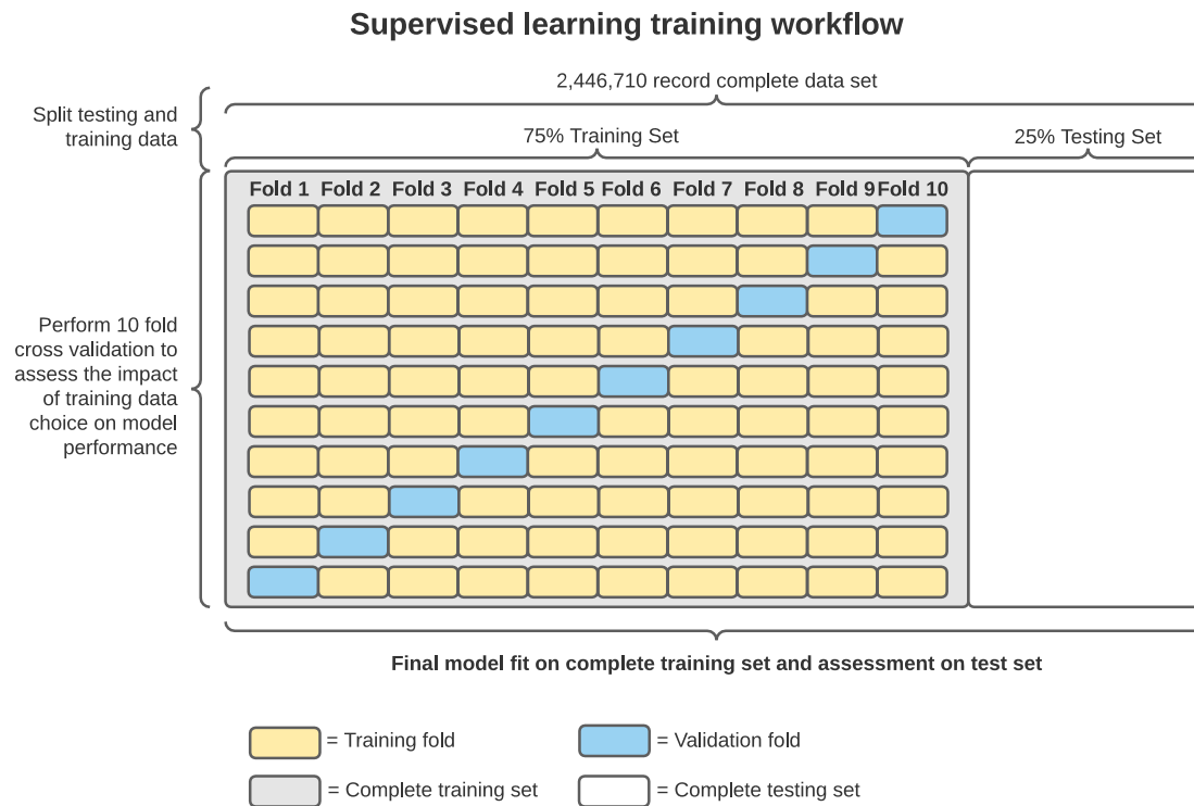
Figure S1. Data partitioning for cross validation
