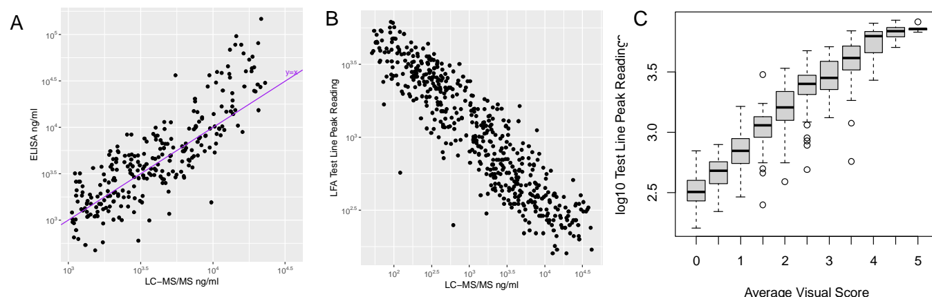
Figure 1: (A) Correlation between ELISA vs LC-MS/MS, for samples with a TFV concentration within the ELISA quantitative of 1,055 ng/mL to 23,000 ng/mL, on log-log axes. The ideal ‘ y=x ’ line is shown for reference. (B) Correlation between LFA test line (optical reader) with LC-MS/MS, on log-log axis. (C) Correlation of intensity of LFA test line (measured by the optical reader) with visual score, on log10 y-axis.
