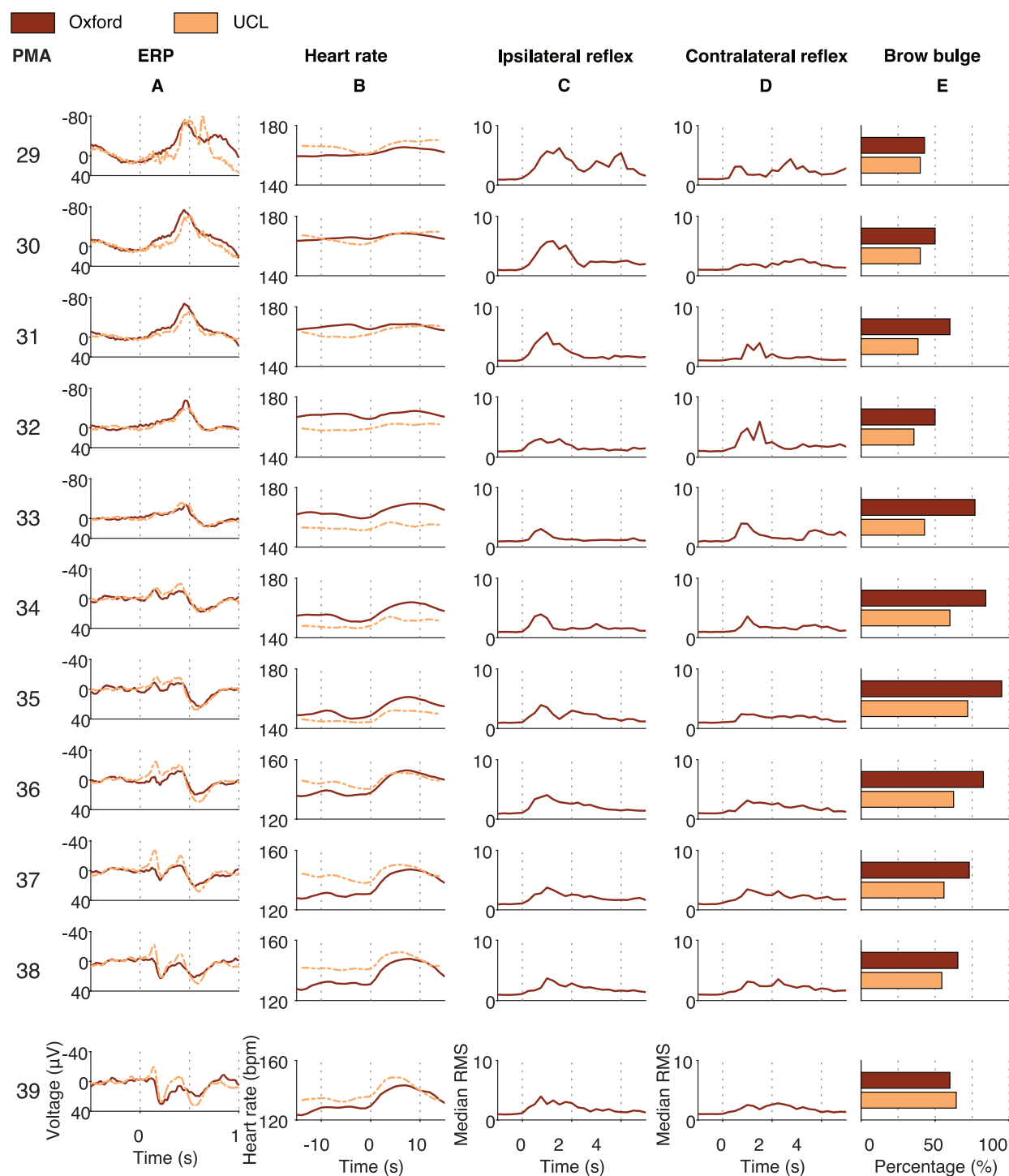
Figure 3. Noxious-evoked ERP, heart rate, ipsilateral reflex, contralateral reflex and brow
