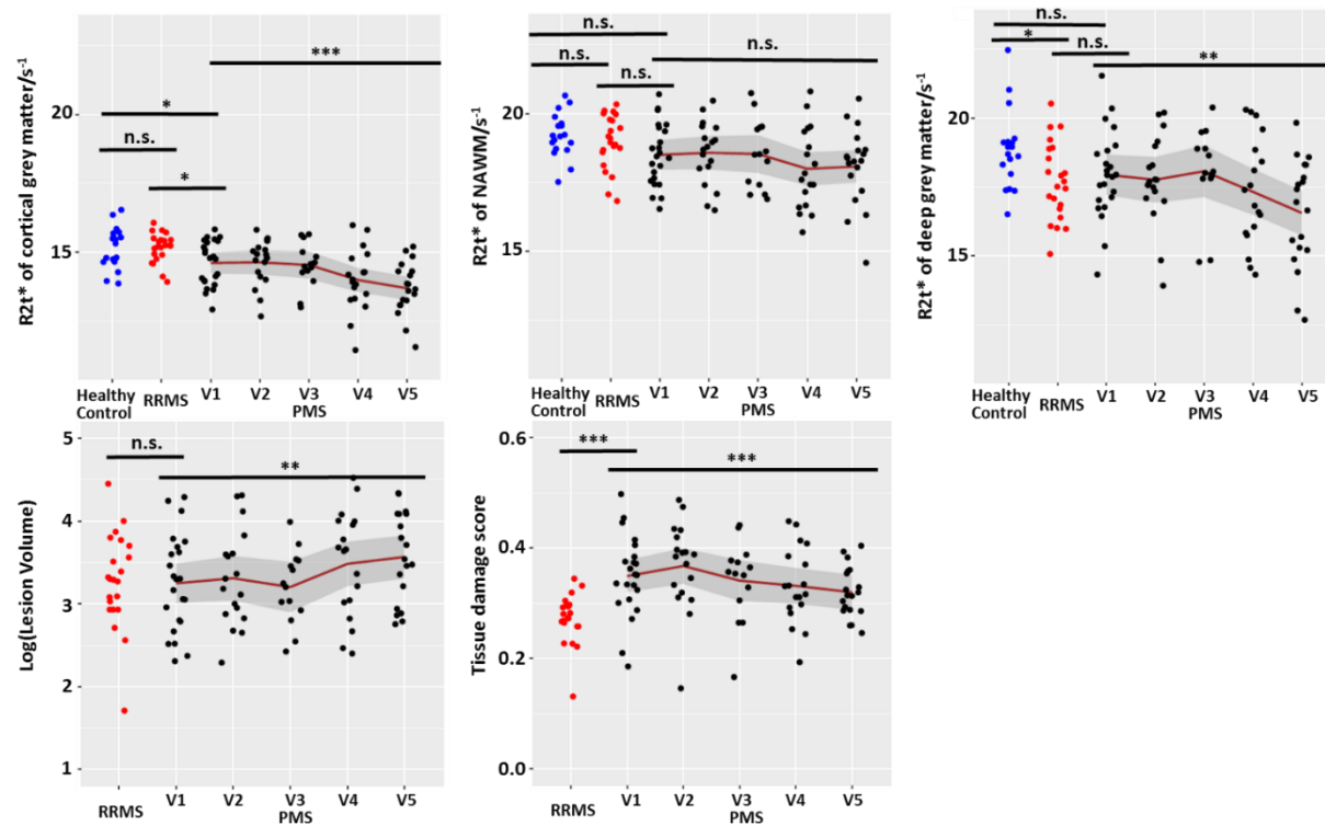
Figure 2. Longitudinal R2t*, lesion volume and tissue damage score measurements for non-relapsing PMS subjects compared with healthy control and RRMS measurements. The longitudinal PMS cohort showed significant decreasing of R2t* (greater microstructural tissue damage) in cortical GM and deep GM over five imaging sessions, performed nine months apart. R2t* of cortical GM and deep GM in visit five were significantly different from R2t* in visit one ( p < 0.001 and p < 0.01 , respectively). The R2t* measurements in GM of PMS subjects at baseline were significantly lower than healthy control and RRMS cohorts ( p < 0.05 ). Lesion volume of PMS subjects increased over four years. Specifically, lesion volume in visit five was significantly higher than the lesion volume in visit one ( p < 0.01 ). Tissue damage score declined over the last four visits, which is likely due to the decrease of R2t* in NAWM, making the differences between R2t* in NAWM and lesion volume smaller. The line represents the mean value and the gray area represents the standard error. One-way ANOVA with repetitive measurements was used to compare the difference between visit one and each subsequent visit of the PMS group. Dunnett test was used to correct for multiple comparisons. One-way ANOVA was used to compare the healthy control, RRMS and baseline visit one of the PMS group. Tukey test was used to correct for multiple comparisons. *** p < 0.001 , ** p < 0.01 , * p < 0.05 , n.s. p > 0.05 .
