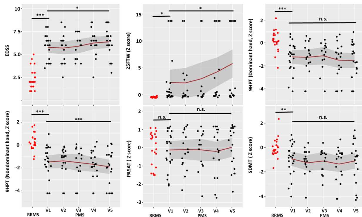
Figure 1. Clinical assessments of the PMS cohort over four years. Compared with the PMS cohort at baseline, the RRMS cohort (red dots) showed significantly better clinical test scores. EDSS, 25-foot walk and 9-hole peg test showed an increasing trend of disability and motor dysfunction for the longitudinal PMS cohort over five imaging sessions, suggesting MS progression within that group. For EDSS, 25FTW and 9HPT (non-dominant hand), there were significant differences between scores in visit five and visit one ( p < 0.05 , p < 0.05 , p < 0.001 , respectively). 25FTW, 9HPT, PASAT and SDMT were converted to Z scores. Each dot represents one subject. The gray area represents the standard error. One-way ANOVA with repetitive measurements was used to compare the difference between visit one and each subsequent visit of the PMS group. Dunnett test was used to correct for multiple comparisons. Two-sample t-test was used to compare the RRMS cohort to the first visit of PMS group. *** p < 0.001 , ** p < 0.01 , * p < 0.05 , n.s. p > 0.05 .
