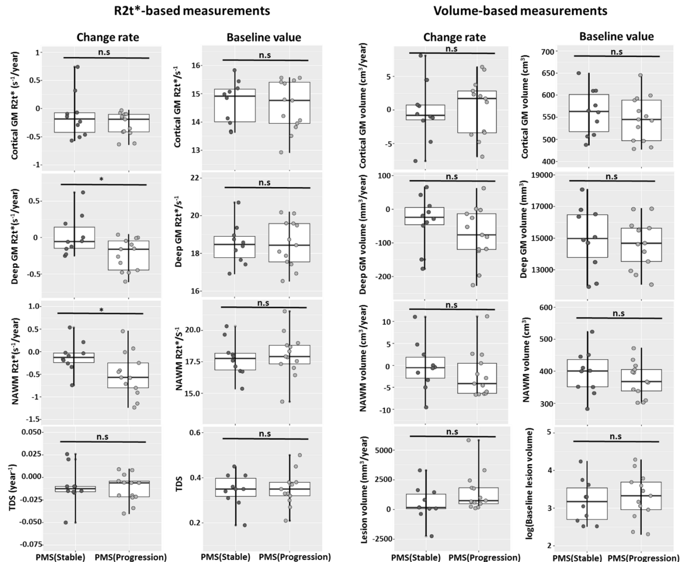
Figure 3. Rate of R2t* decline in NAWM and deep grey matter was faster in PMS subjects with clinically defined progression than in stable PMS subjects. Thirteen PMS subjects showed clinically defined progression, whereas ten subjects were stable on clinical tests. Each dot represents one subject. Each row corresponds to an imaging biomarker. The first and third columns of graphs show rate of change and the second and fourth columns show the baseline values. Rate of change of R2t* in deep grey matter and NAWM were significantly faster in PMS with clinical progression, whereas rate of change in lesion tissue damage score, lesion volume, NAWM volume and deep GM atrophy were nominally greater in the PMS group with clinical progression group than the stable group, but did not reach statistical significance. * p < 0.05 , n.s p > 0.05 .
