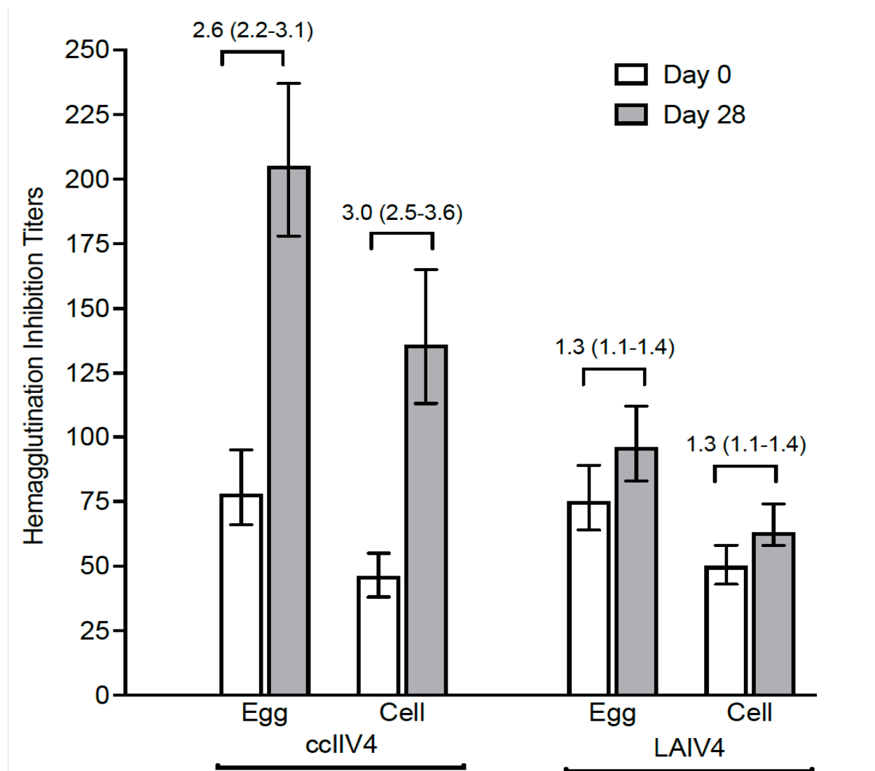
Figure 2. Pre- and post-vaccination GMT hemagglutination inhibition (HAI) assay titers by vaccine type for A/H3N2-A/Kansas egg and cell grown viruses. Data are day 0 (white) and day 28 (gray) with 95% confidence Intervals (CI), GMFR with 95% CI is shown horizontally above bars. Within each vaccine type, egg grown antigens were higher than cell grown at days 0 and 28 ( p < 0.001 ), but the GMFR did not differ between egg and cell. Between vaccine types, HAI titers at day 28 and GMFR were lower for LAIV4 for each respective antigen ( p < 0.0001 ).
