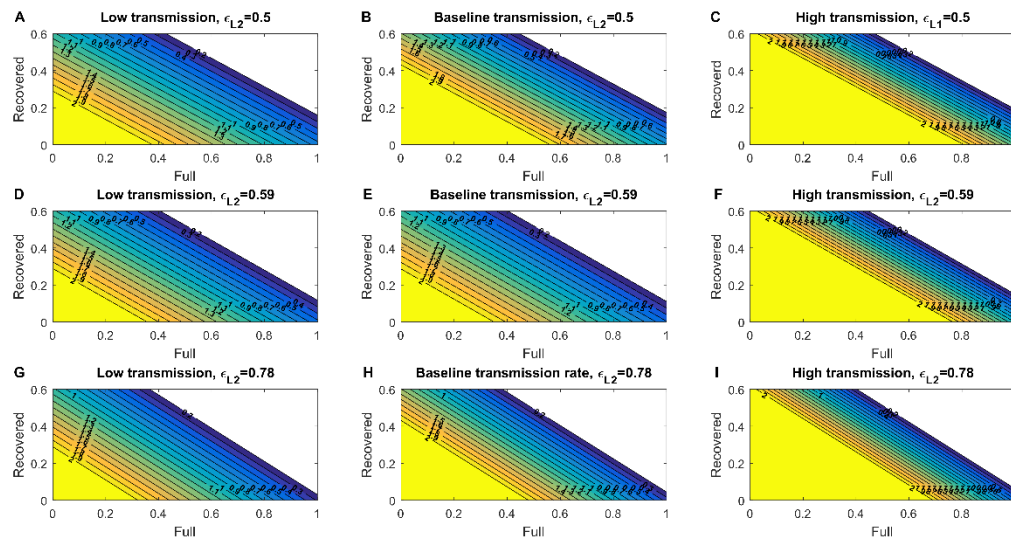
Figure 2. Control Reproduction number for symptomatic transmission considering full immunity and recovered individuals. The assumed vaccine effectiveness ( \epsilon_{L2} ) parameter under each scenario is denoted on top of each panel and are inferred based on real-world data of individuals receiving two doses of the BNT162b2 vaccine [9]. The heatmaps in left row consider a low transmission rate; the heatmaps in the center row panels consider a baseline transmission rate; and the heatmaps in the right row panels consider a high transmission rate.
