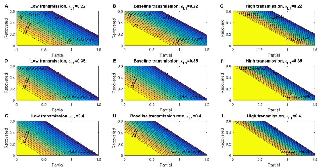
Figure 4. Control Reproduction number for symptomatic transmission considering partial immunity and recovered individuals. The assumed vaccine effectiveness ( \epsilon_{L1} ) parameter under each scenario is denoted on top of each panel and are inferred based on real-world data of individuals acquiring partial immunity as those induced by one dose of the BNT162b2 vaccine [9]. The heatmaps in left row consider a low transmission rate; the heatmaps in the center row panels consider a baseline transmission rate; and the heatmaps in the right row panels consider a high transmission rate.
