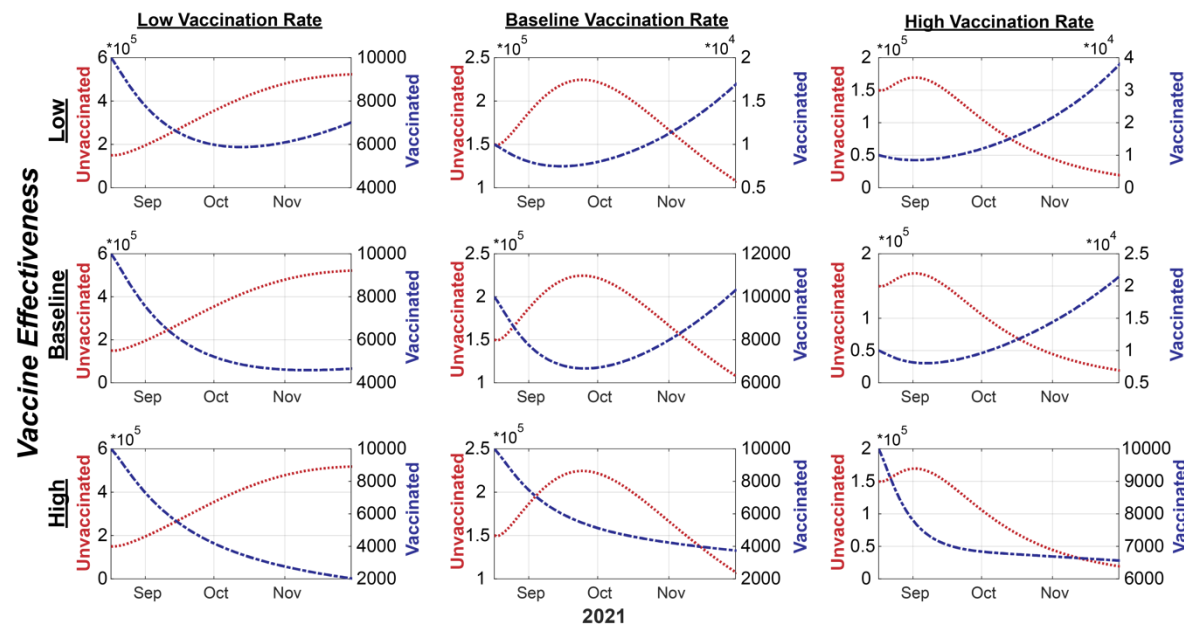
Figure 2. Modelled projections of symptomatic infections in unvaccinated and vaccinated subpopulations under different vaccination rates and vaccine effectiveness. The case counts of the unvaccinated individuals are depicted by the red line and the unit labels on the left-side y-axis, whereas the infected, vaccinated (breakthrough) cases are depicted by the blue line and the unit labels on the right-side y-axis.
