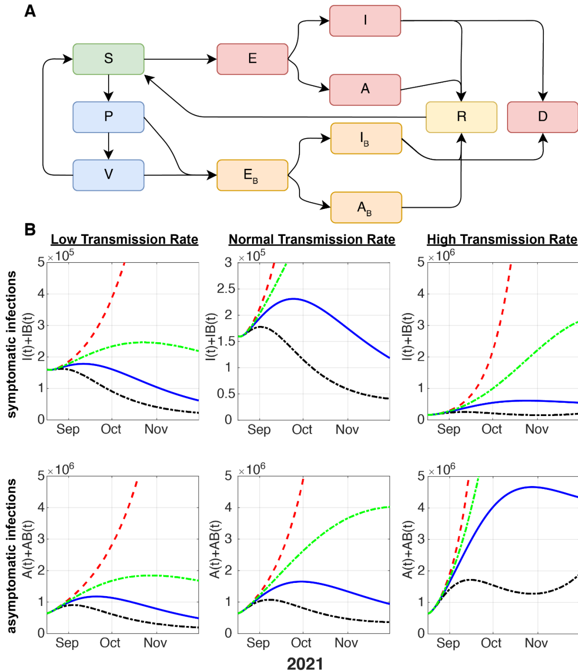
Figure 1. Schematic of the model considering vaccinated vs. unvaccinated individuals and projection of newly infected symptomatic and asymptomatic cases. (A) Flow dynamics of the mathematical model. S: susceptible, P: partial immunity (one vaccine dose), V: full immunity (two vaccine doses). E: unvaccinated, exposed. I: unvaccinated, infected and symptomatic, A: unvaccinated, infected, asymptomatic. E_B : vaccinated ( \geq 1 dose), exposed. I_B : vaccinated ( \geq 1 dose), infected, and symptomatic ("breakthrough cases"). A_B : vaccinated ( \geq 1 dose), infected and asymptomatic. R: recovered. D: deceased. (B) Modelled dynamics of the new infections that are symptomatic (top row) and asymptomatic (bottom row) from the SARS-CoV-2 delta variant considering different vaccination rates. The red line presents zero vaccination; the green line represents a 50% decrease in VR; the blue dotted line means baseline VR and the black dotted line denotes 200% VR.
