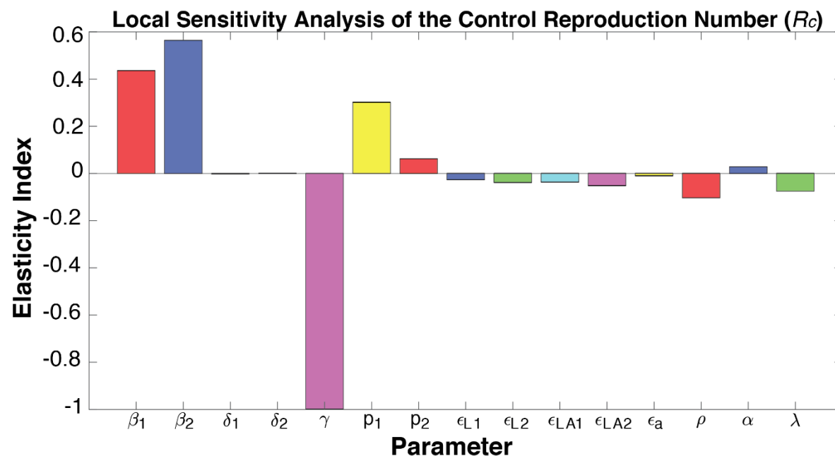
Figure 3. Elasticity index showing each modelled parameter's effect on the control reproduction number as determined in the local sensitivity analysis. For each column, a positive value represents an increase of the parameter is associated with an increment in the control reproduction number, whereas a negative value means a decrease.
