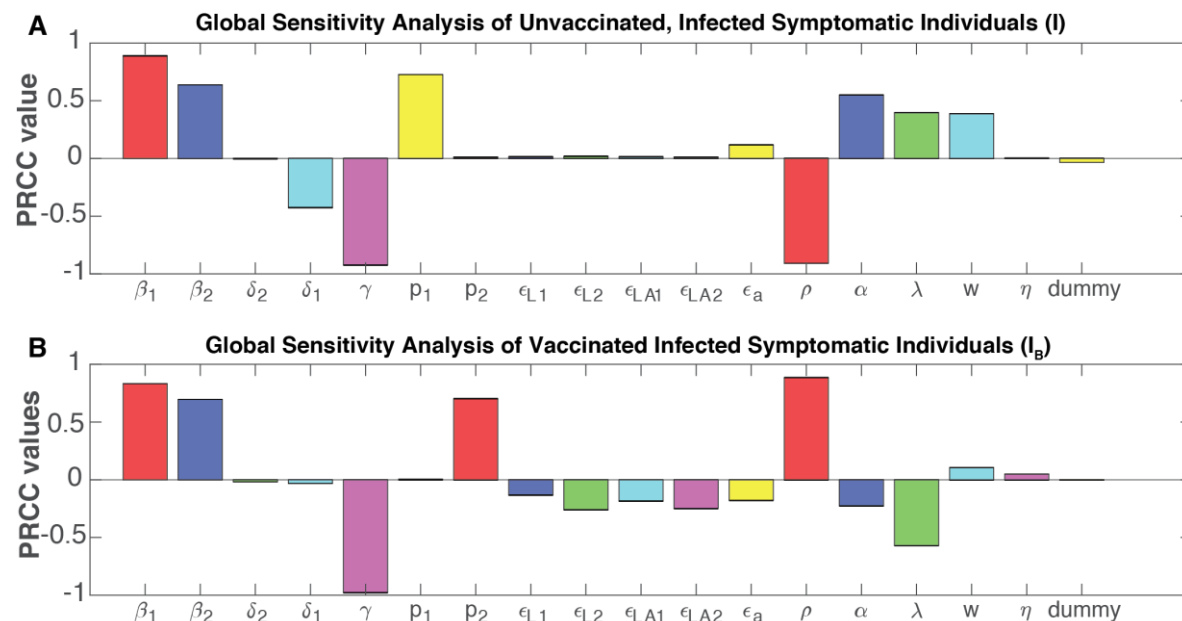
Figure 4. Global sensitivity analyses of the parameters correlated with the symptomatic infections in (A) unvaccinated, and (B) vaccinated individuals. The relationship between each parameter and the infected subpopulation is measured by the Partial Rank Correlation Coefficient (PRCC); a positive PRCC indicates an increase in the parameters is correlated with an increase of the said sub-population, and a negative PRCC vice versa. The significance level of each PRCC is indicated in Fig. S6.
