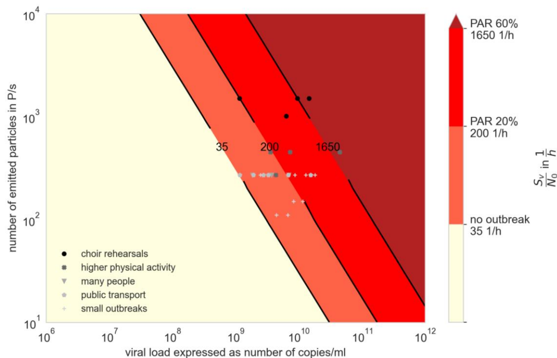
Figure 3: Virus Factor (VF) for different viral loads and particle emission rates with N_0=100 viral copies, the attack rates found in the investigated outbreaks are shown with the different colors; the markers show the amount of virus factor at assumed mean particle emission rate of the related activity according to Figure 2.
