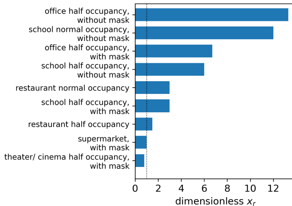
Figure 6: comparison of the risk factor x_r for different everyday life situations: 0,5 hour stay in a supermarket, wearing a mask as reference
