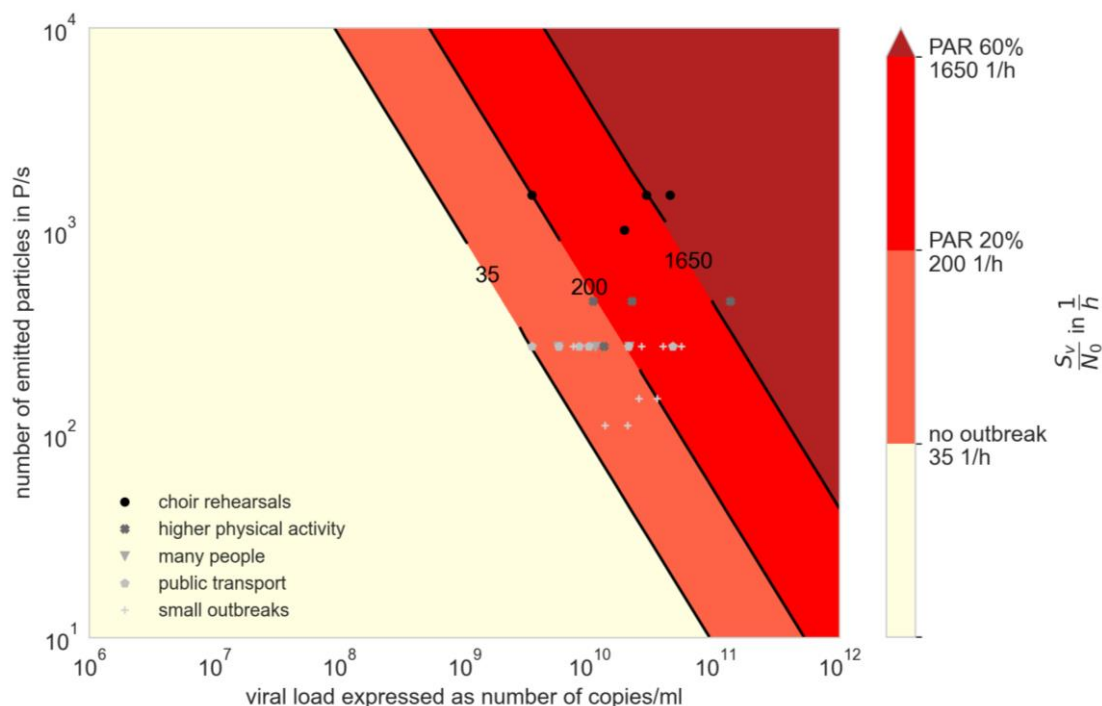
Figure 4: Virus Factor (VF) for different viral loads and particle emission rates with N_0=300 viral copies, the attack rates found in the investigated outbreaks are shown with the different colors; the markers show the amount of virus factor at assumed mean particle emission rate of the related activity according to Figure 2.
