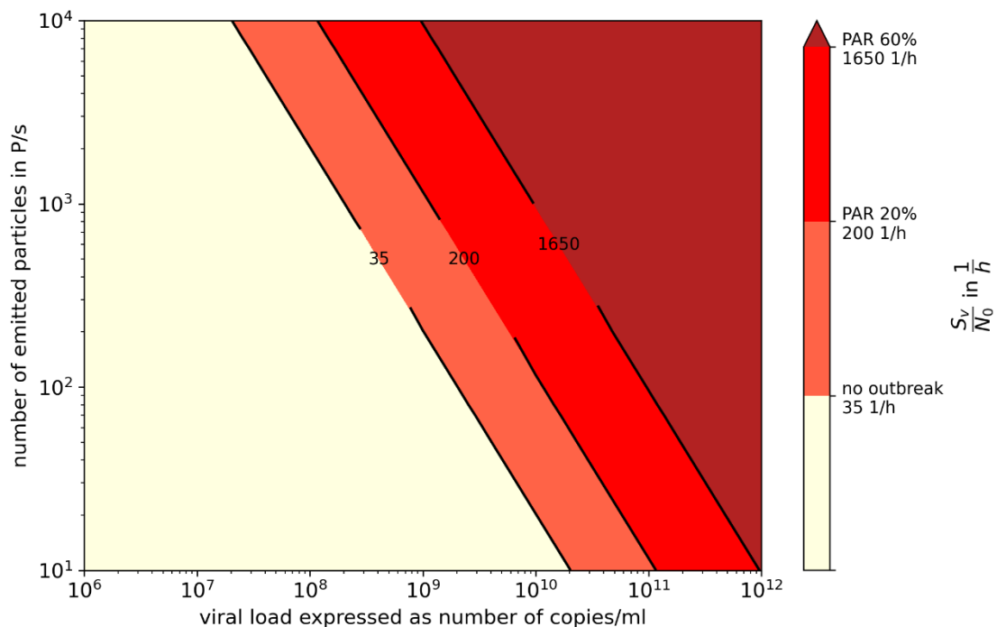
517 Figure 8: viral emission for different viral loads and particle emission rates with N_0=67 viral copies, the attack rates found in 518 the investigated outbreaks are shown with the different colors
