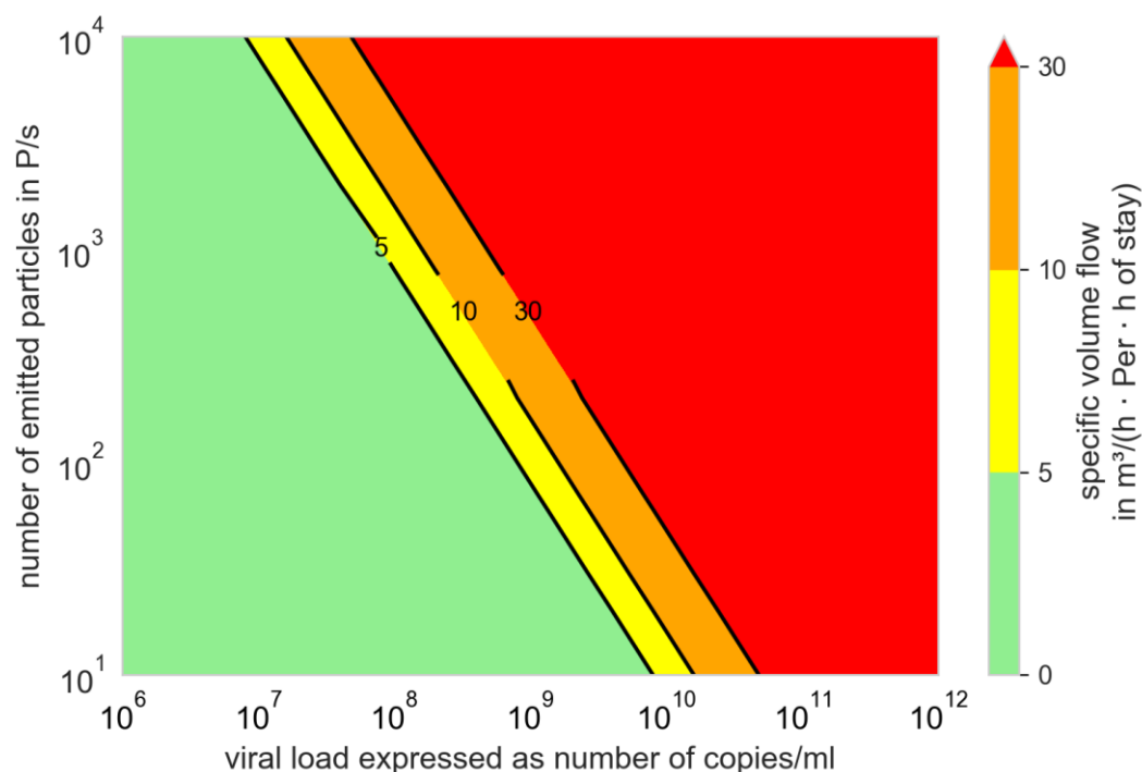
Figure 5: specific volume flow depending on the number of emitted, particles and the viral load to limit the number of newly infected persons to one, N_0=100 viral copies, f_M=1 , Q_{b,in}=Q_{b,e}=0.54m^3/h
