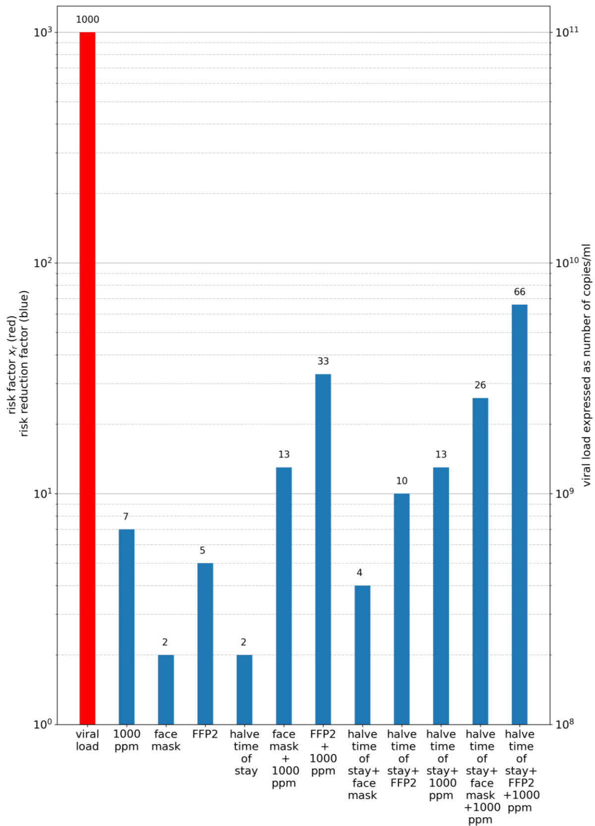
Figure 10: influence of different preventive measures on the risk of an outbreak. The red bar represents the viral load and the resulting risk factor (eq. 37). The blue bars illustrate different combinations of preventive measures in the form of a risk reduction factor (also according to eq. 37).
