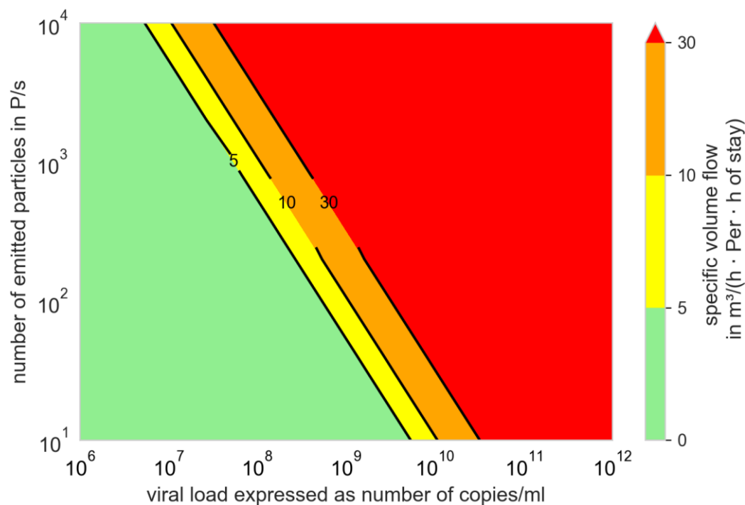
Figure 9: specific volume flow depending on the number of emitted, particles and the viral load to limit the number of newly infected persons to one, N_0=67 viral copies, f_M=1 , Q_{b,in}=Q_{b,e}=0.54\text{m}^3/\text{h}
