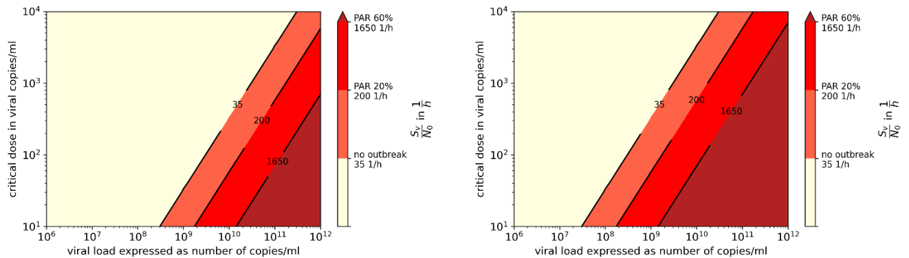
509 Figure 7: Virus Factor for different viral loads and critical doses with a particle emission rate of 100 P/s, (left) and 1,000 P/s 510 (right), the attack rates found in the investigated outbreaks are shown with different colors
