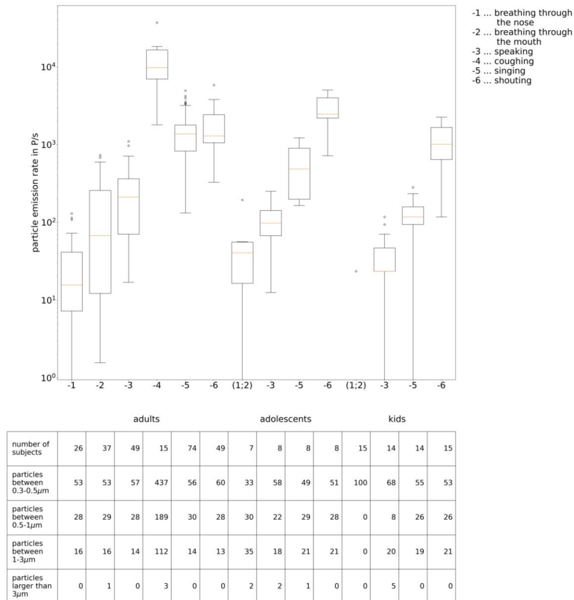
Figure 2: particle emission rates measured by some of the authors, for adults: [31, 36, 32], for adolescents [35] and for children [38]
