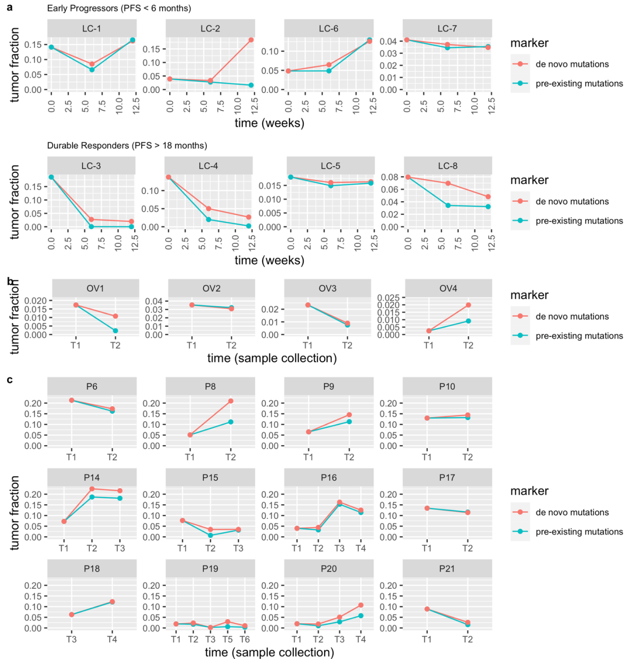
Figure 5. Longitudinal cfDNA monitoring in cancer patients who received treatments. The lines show the tumor fraction in cfDNA during treatment. (a) Tumor fraction in plasma samples of 8 NSCLC patients who received anti-PD-1 immunotherapy. (b) Tumor fraction in serum samples of 4 ovarian cancer patients. (c) Tumor fraction in plasma samples of 12 prostate cancer patients.
