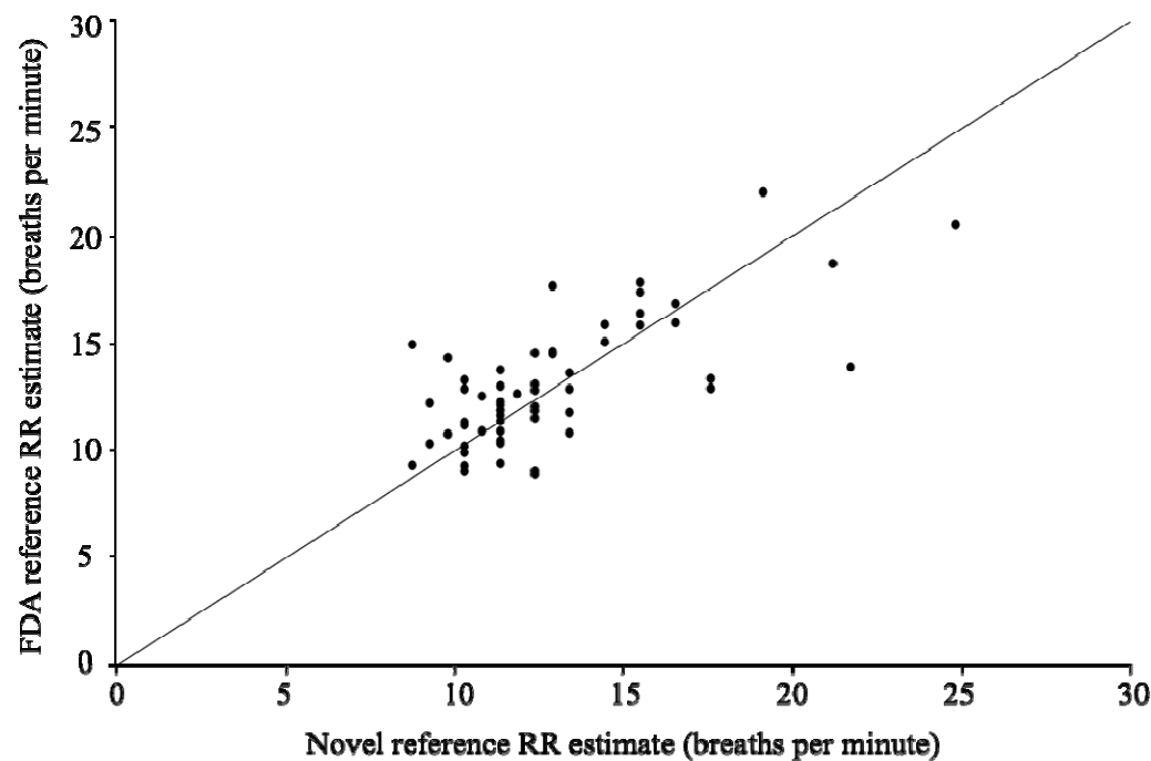
Figure 7. Scatterplot for simultaneous RR estimates provided by the novel reference (x-axis) and FDA-cleared reference (y-axis). The solid line indicates the gradient y=x . Marker size is proportional to the number of observations for each combination of values.
