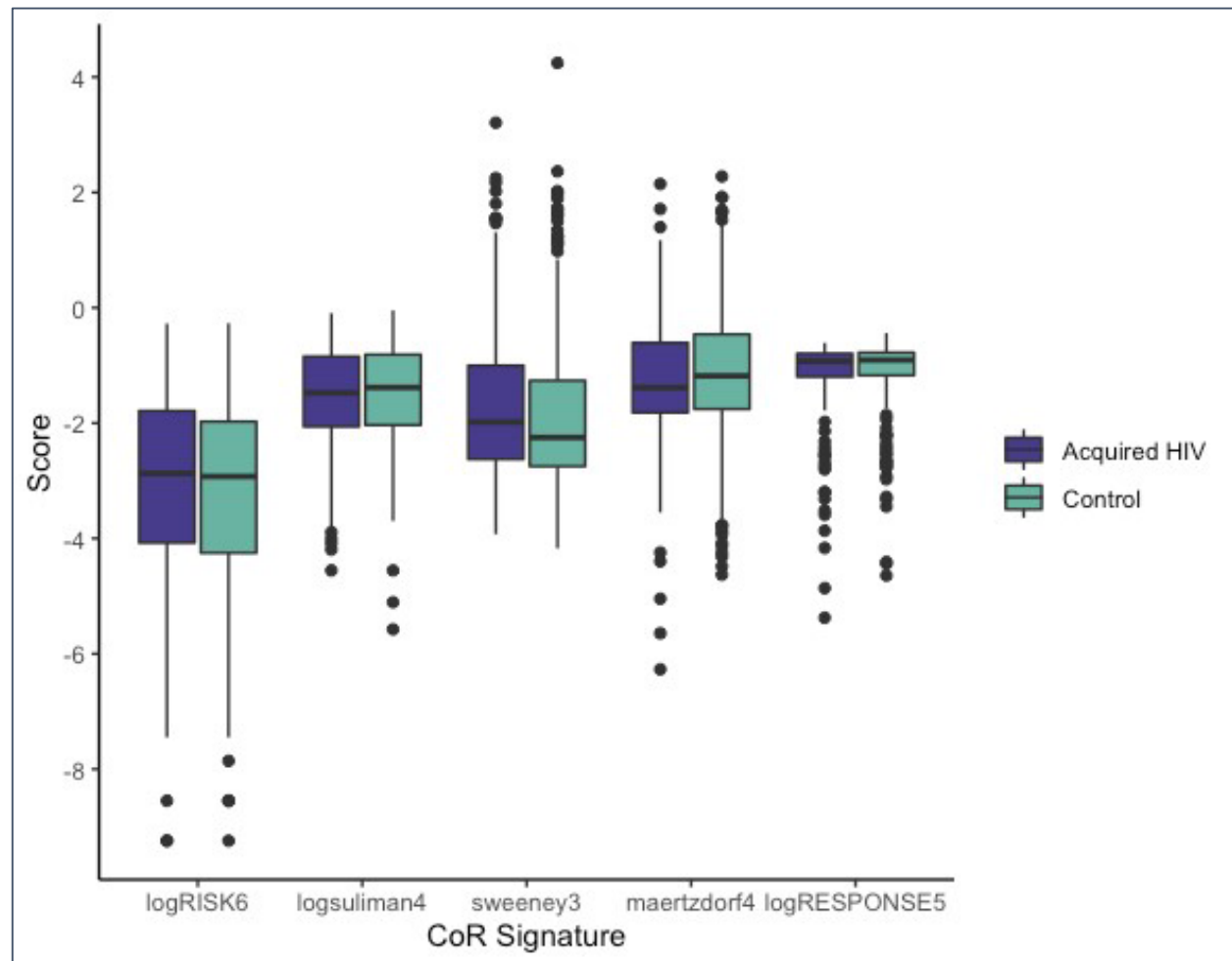
Figure 2: Distribution of 5 TB Correlates of Risk (CoR) scores among participants who subsequently acquired HIV vs controls. Box plots demonstrate median and interquartile range of values, with dots completing the range. RISK6, Suliman4, and RESPONSE5 were \log_{10} transformed as this allowed for the data to be normally distributed and for all scores to be evaluable on a similar scale.
