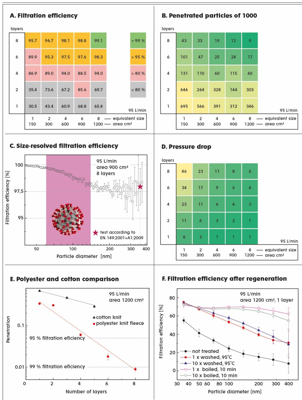
Fig 2. Characteristics of the knit PES fleece fabric used as a filter material.
