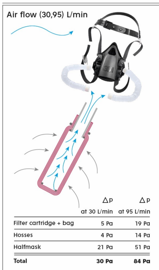
Fig 4. Pressure drop of the filter kit and its components.
