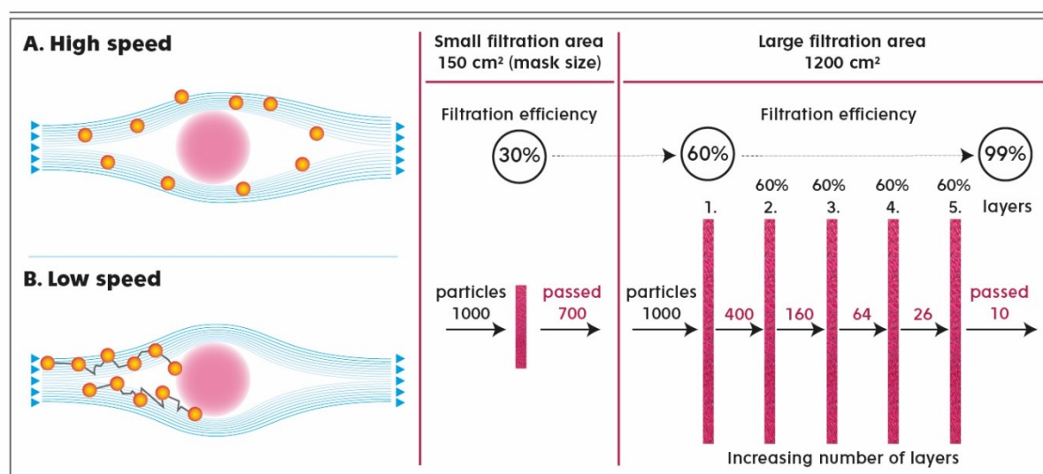
Fig 1. Principle of filtration efficiency enhancement.
