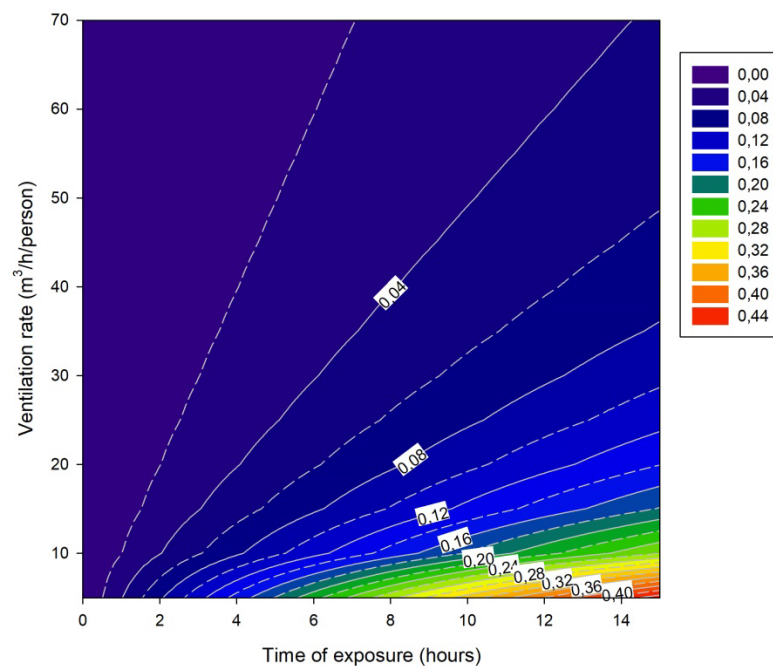
Figure 2: Probability of infection contours as a function of time of exposure and ventilation rate per person assuming a quantum rate of 40 h -1 , an expiratory rate of 0.50 m 3 /h and an infector proportion of 0.01.
