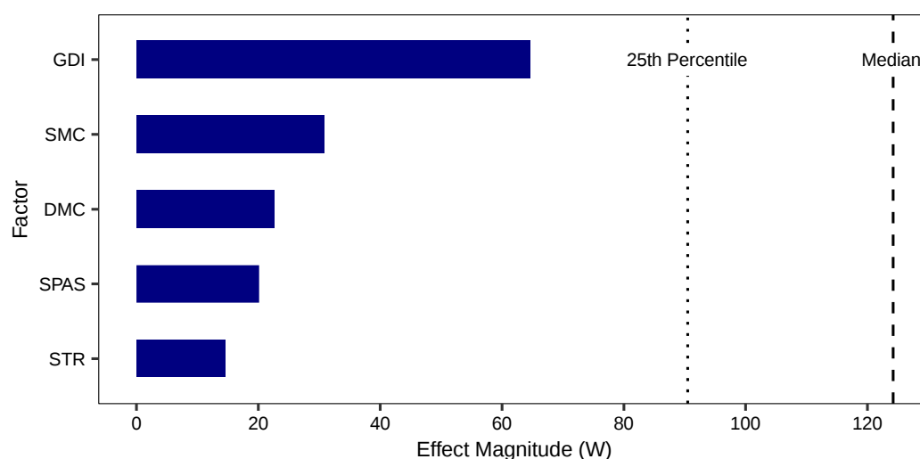
Figure 3. The range of the causal effect for each factor for the middle 95th percentile. The dotted and dashed lines show the 25th percentile and median metabolic power of children included in this study. The total effect of GDI is approximately twice that of SMC and DMC, and more than thrice that of spasticity or strength.
