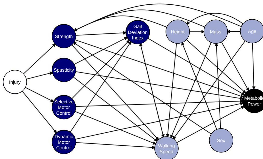
Figure 1. Causal model (portrayed as a directed acyclic graph) of the potential contributors to high metabolic power during walking in children with cerebral palsy (CP). The initial brain injury is colored white to represent an unmeasured factor. Despite being unmeasured, including the initial brain injury helps to simplify the complex relationship between neurological impairments in CP. Blue nodes are factors often treated and measured in the clinic (neurological and physical impairments), so understanding their effects offers a better understanding of their importance in treating metabolic power. Metabolic power, colored in black, is the outcome of interest. Gray variables are potential confounders.
