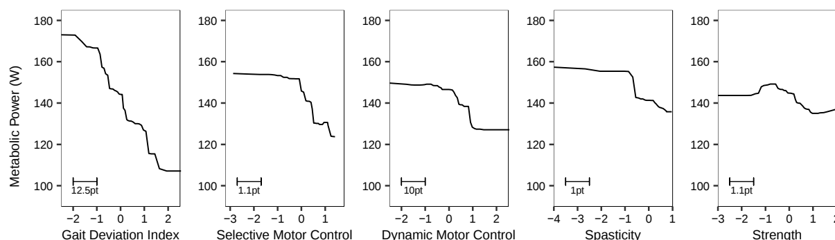
Figure 2. Accumulated local effects plot of the total causal effects of gait deviation index, selective motor control, dynamic motor control, spasticity, and strength on metabolic power with 95% bootstrapped confidence intervals. These plots represent the average change in metabolic power that can be expected with a change in the x-variable. X-axis variables are normalized as z-scores, where increasing or more positive scores indicate a lesser severity of impairment (i.e., more typical gait, more coordinated, less spastic, stronger). Rug plots along the x-axis display the distribution of scores for each impairment. The bottom right scale indicates how large a single standard deviation is with respect to original units.
