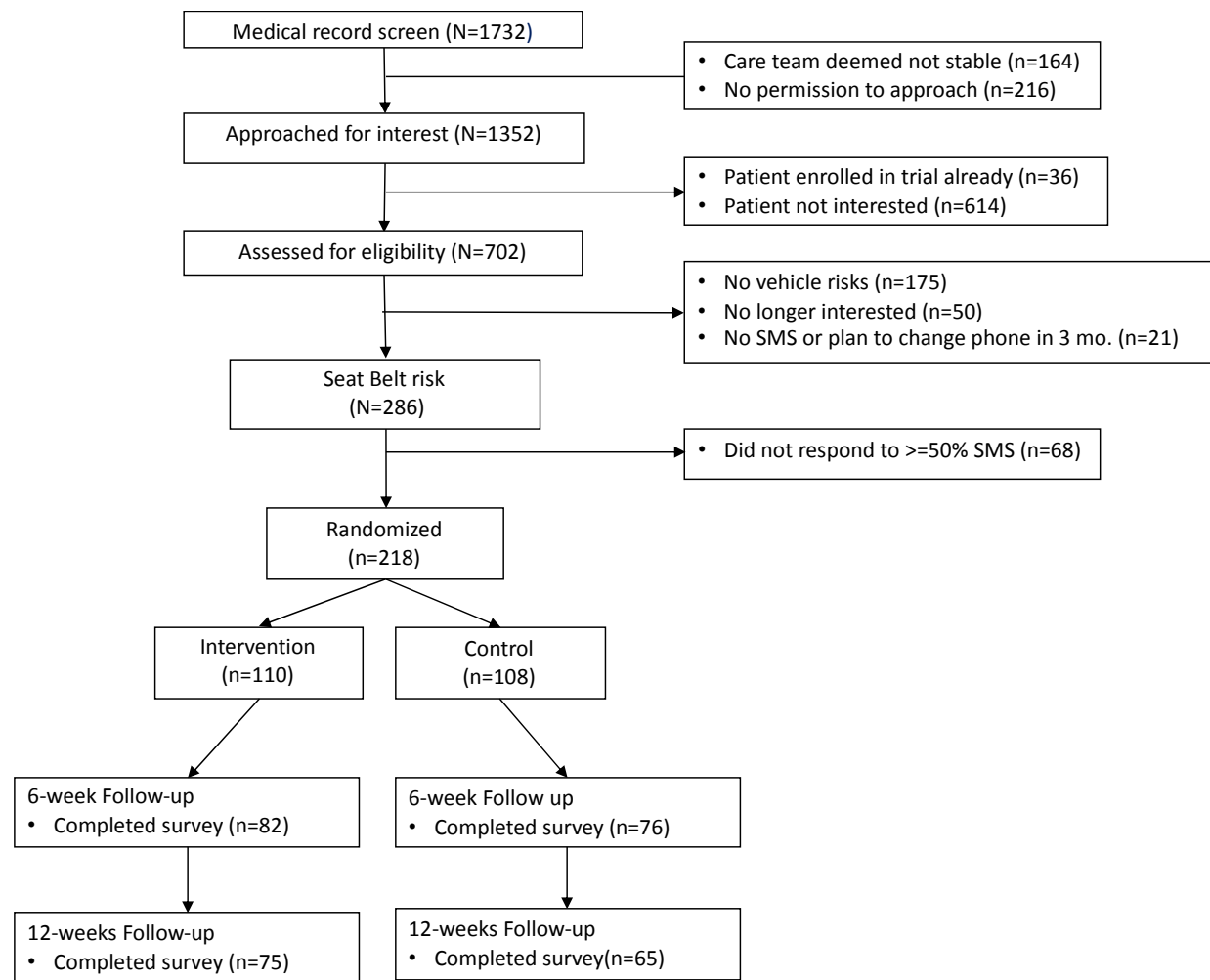
Figure 1: CONSORT Diagram
