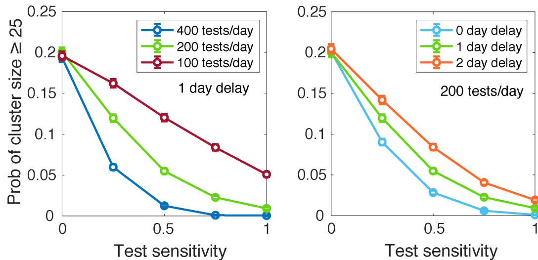
Fig 3: Results of a Monte Carlo simulation of infection transmission on a network of 1600 individuals. We track the probability that a single starting infection seeds a cluster of 25 or more infections. We compare a baseline protocol that has a capacity of 200 tests per day and a delay in reporting of one day (green), with variations having higher or lower capacities or delays (see legend). Error bars represent SEM values over 5000 replicate simulations.
