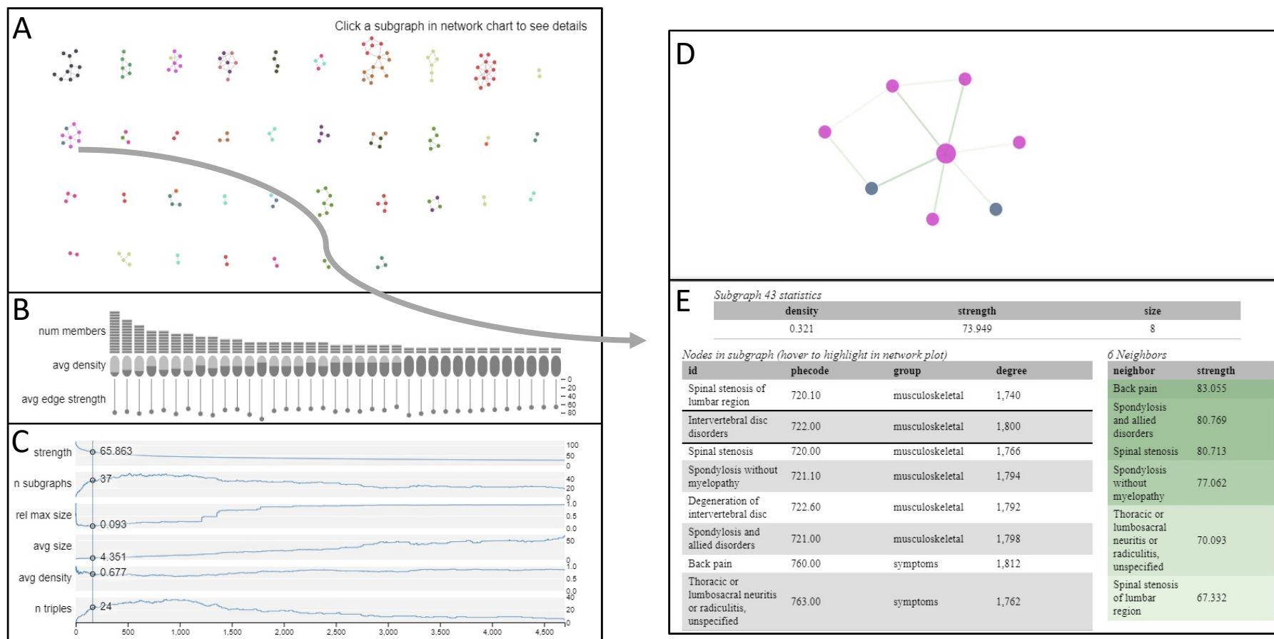
Figure 1: Interactive visualization of subgraph clustering results with current threshold set at the optimal threshold according to the smallest-largest rule
