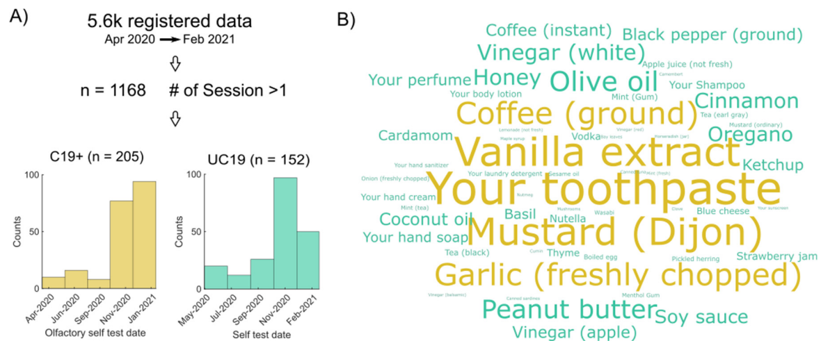
Figure 1. Data, self-test date density, and odors. A) Total number of individuals and the date range of data registration from which we included only individuals with more than one session of data registration. We pseudo-randomly sampled from unidentified COVID-19 status (UC19) cohort to match the population distribution of
