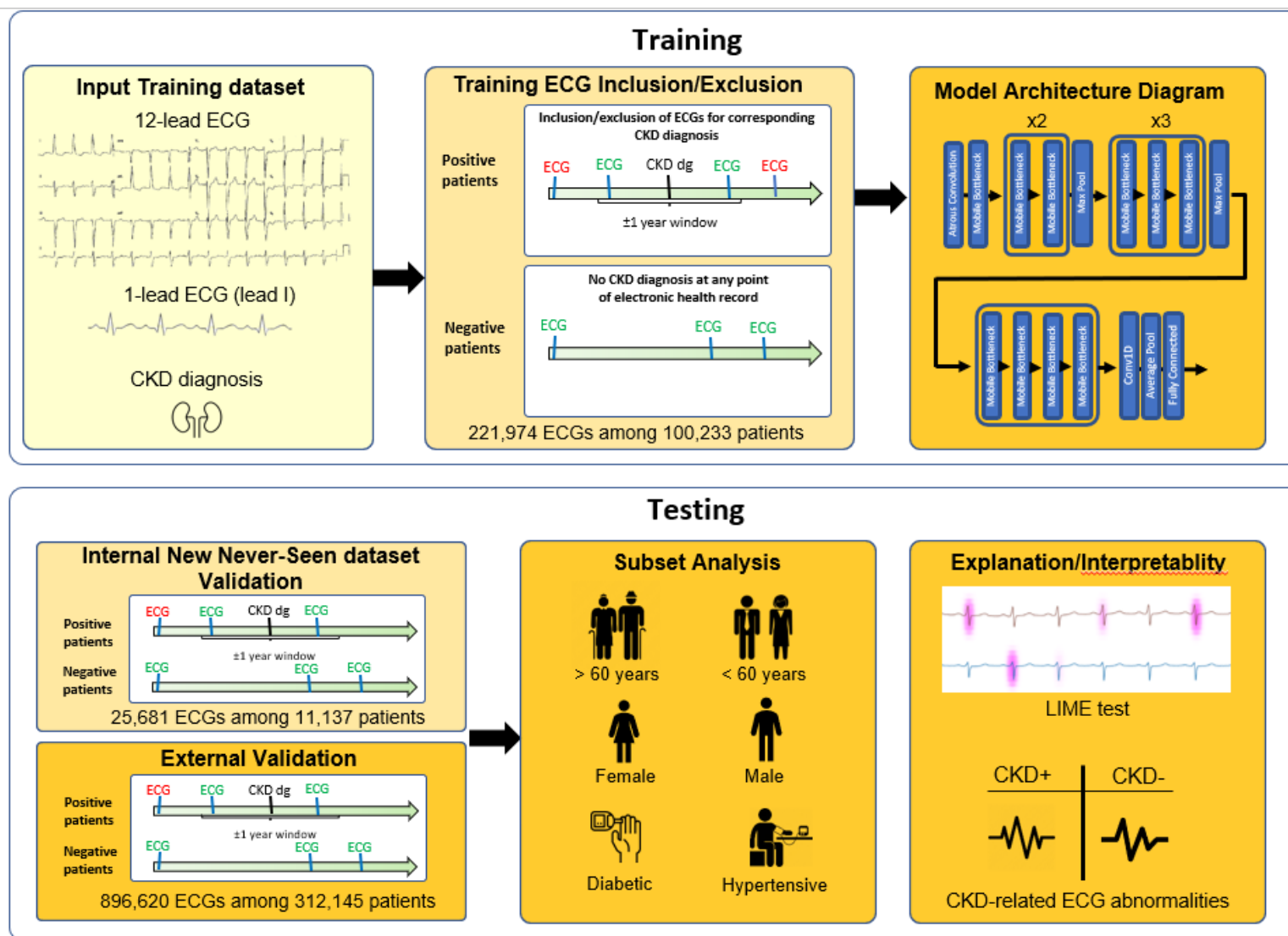
Figure 2. Schematic illustration of deep learning model training, testing, and validation. CKD=Chronic kidney disease.
