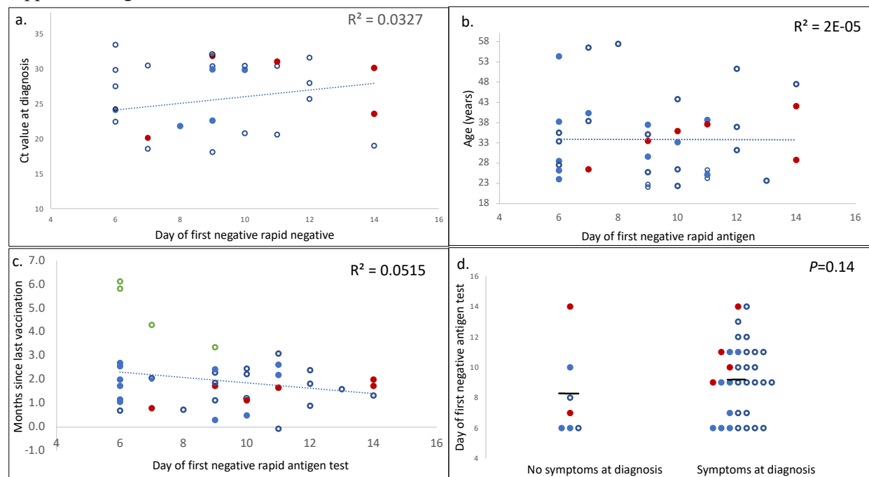
Supplement Figure 1. Relationship between days to first negative RAT and (a) Ct value at diagnosis, (b) participant age, (c) months since last vaccination, and (d) the presence/absence of symptoms at time of diagnosis. Each point represents a single individual in the study. Blue filled circles = individuals who had a sample taken for viral culture and were culture negative. Red filled circles = individuals who had a sample taken for viral culture and were culture positive. Blue open circles = all other individuals. In (c), the four individuals who had been vaccinated but not boosted are shown in green. P-value in (d) was calculated using the student-t test.
