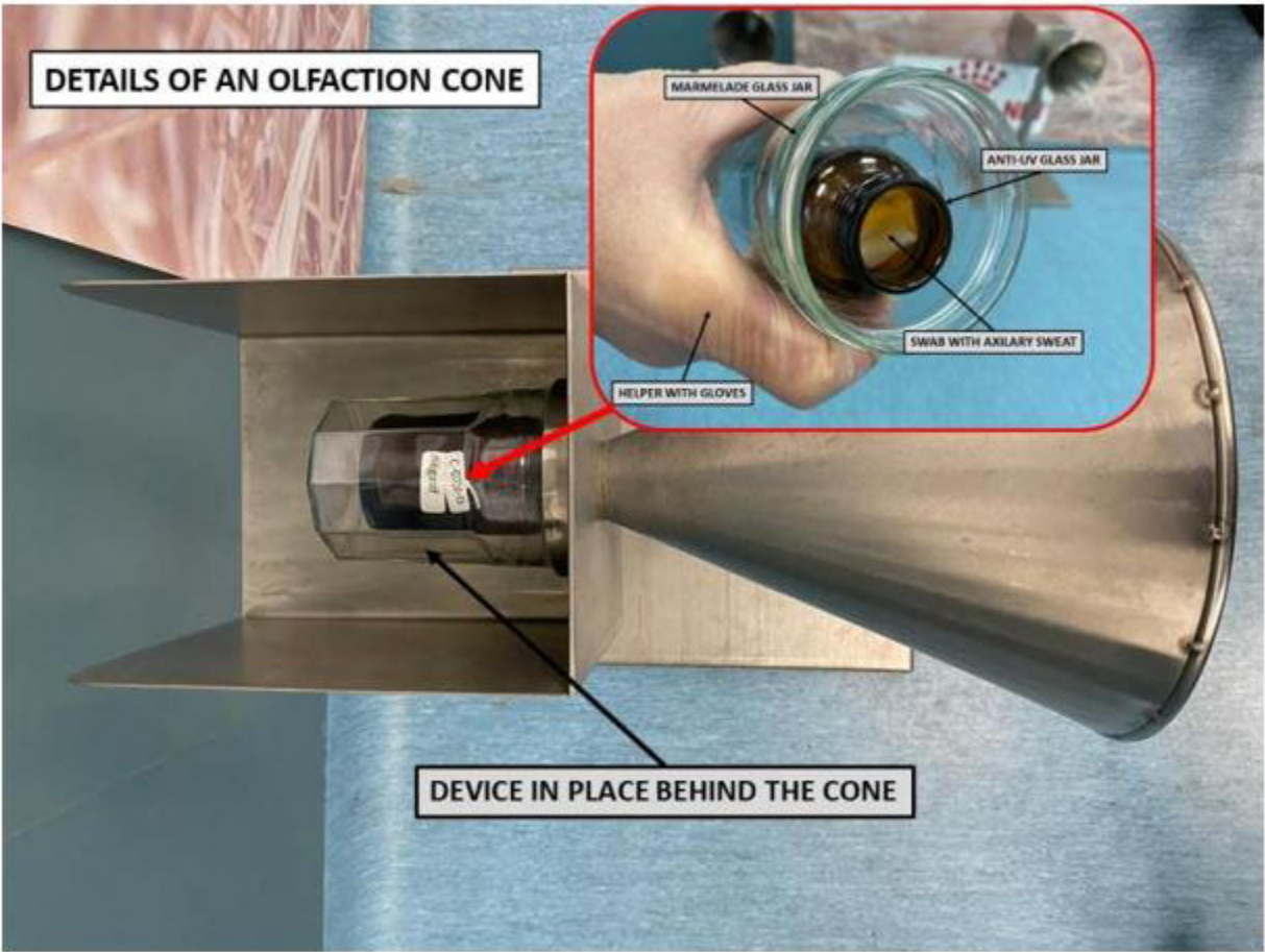
Figure 1B: Details of an olfaction cone, with a double-protected sample and no possibility of direct contact with the dog
