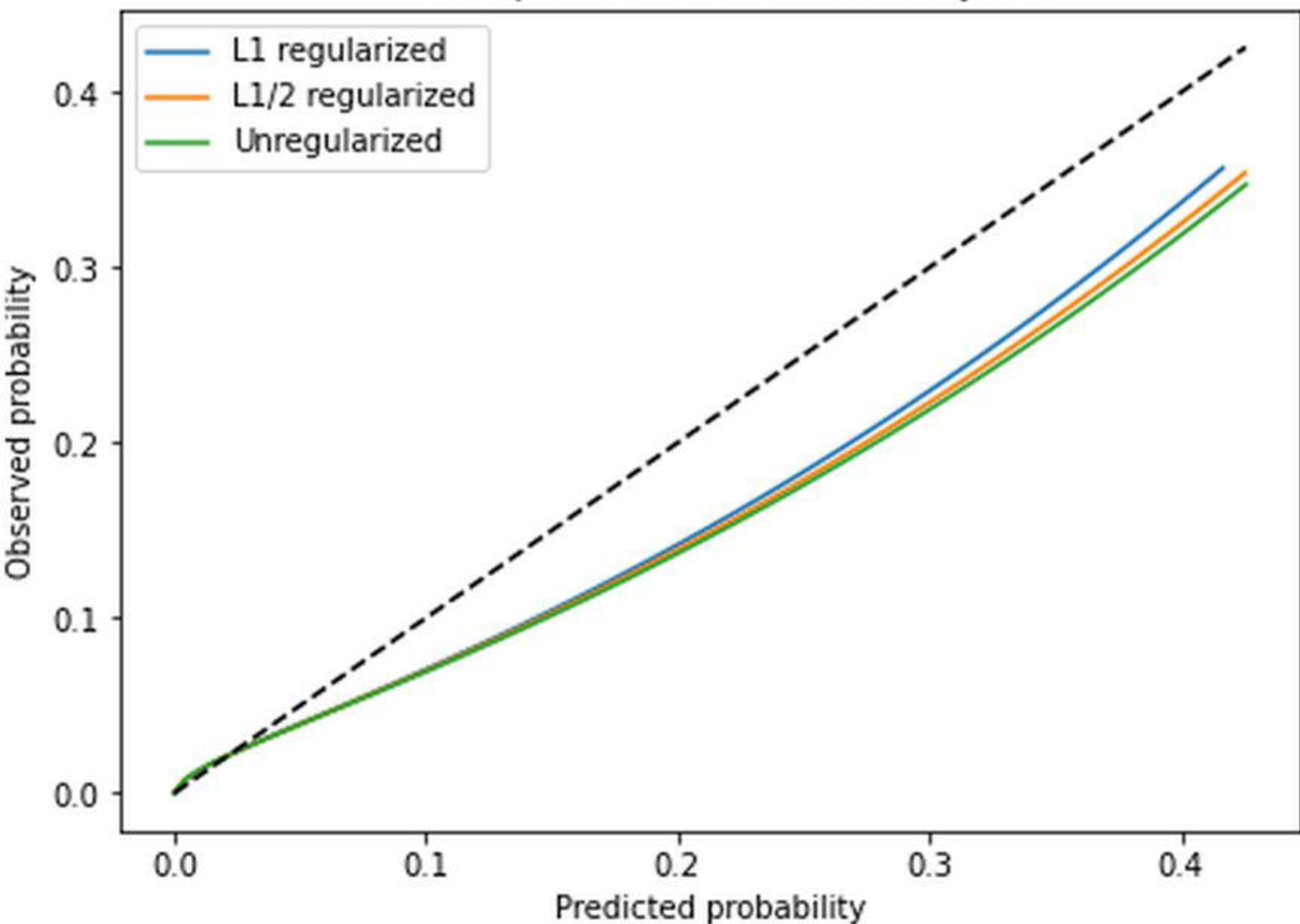
Smoothed calibration curve of survival probabilities at t \leq 1.00 years
