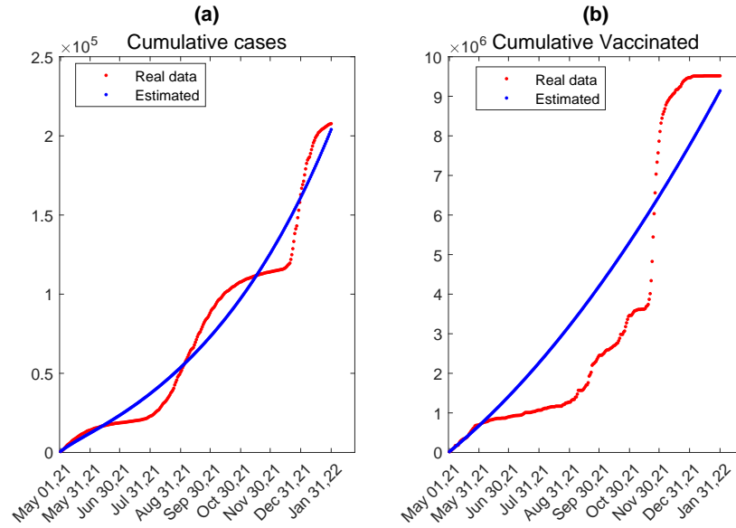
Figure 3: The fitted data to the reported cumulative cases (panel (a)) and cumulative vaccinated (panel (b)) using the model (2) for Ethiopia from May 01, 2021 to January 31, 2022.
