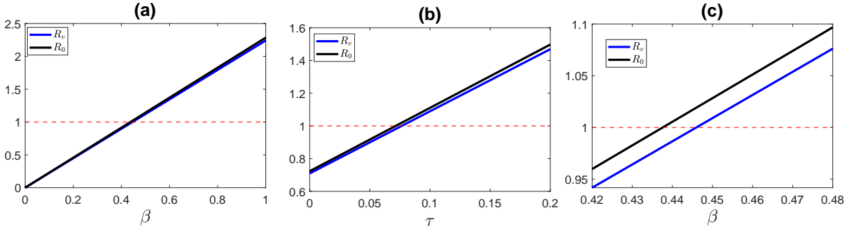
Figure 5: Variation of R_v with respect to : the transmission rate \beta , panel (a) and infectivity factor of asymptomatic individuals \tau , panel (b). Panel (c) shows the zoom plot of panel (a). The red dotted line is used to mark the line at one. Other parameter values are given in Table 2.
