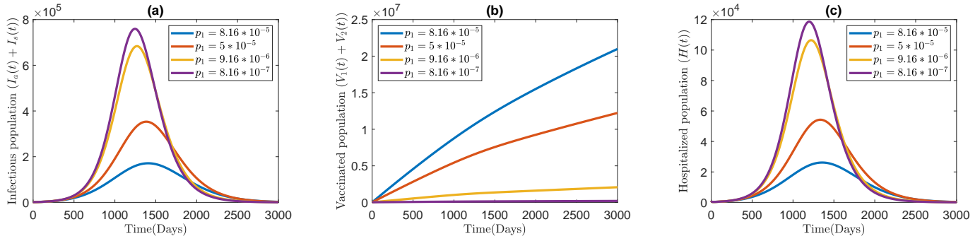
Figure 8: The impact of the first dose vaccination rate p_1 : on the dynamics of infectious population, panel (a), vaccinated population, panel (b), and hospitalized population, panel (c). Other parameter values are given in the Table 2.
