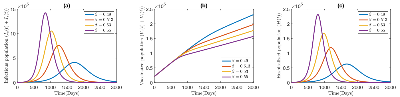
Figure 7: The effect of transmission rate \beta . Panel (a): infectious population I_a(t) + I_s(t) , panel (b): Vaccinated population, V_1(t) + V_2(t) , and panel (c) hospitalized individuals. Other parameter values are given in the Table 2.
