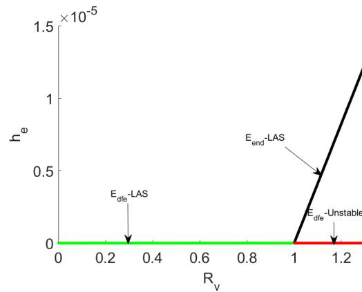
Figure 6: Transcritical bifurcation of model (2) when R_v = 1 .
