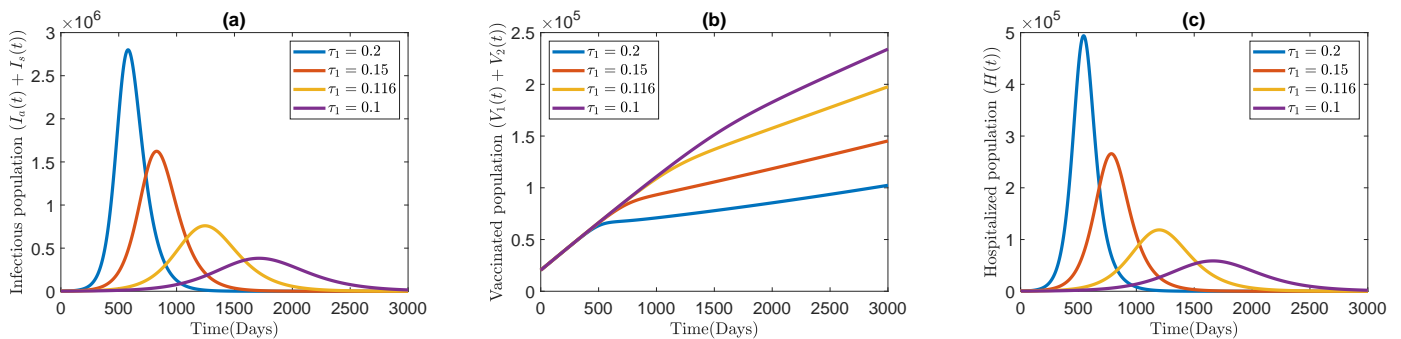
Figure 9: The impact of the infectivity coefficient of asymptomatic population, \tau_1 on the dynamics of infectious population, panel (a), total vaccinated population, panel (b), and hospitalized population, panel (c). Other parameter values are as in the Table (2).
