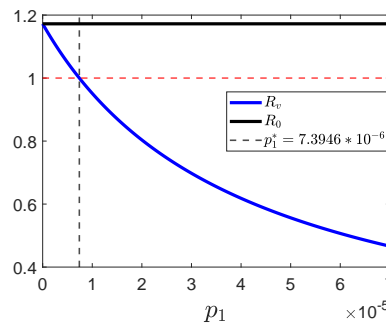
Figure 2: The role of the vaccination rate p_1 on the control reproduction number R_v and the basic reproduction number R_0 . The red broken line is used to mark the horizontal line at 1. p_1^* is calculated using the parameter values in the Table 2.
