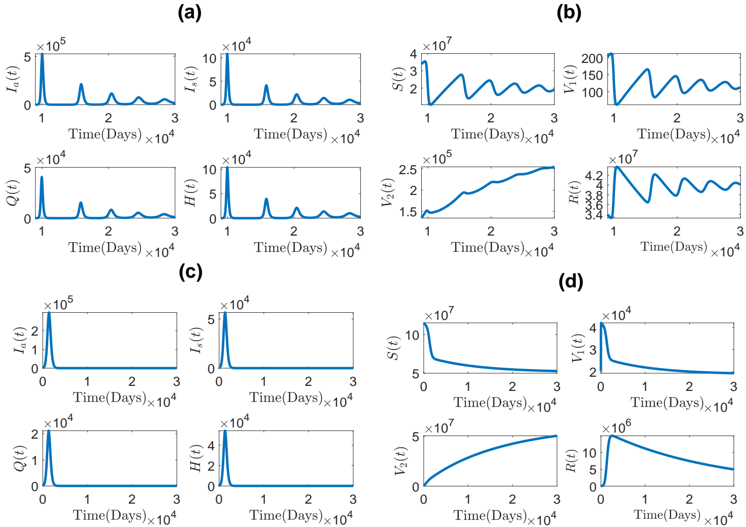
Figure 4: Local stability of the endemic equilibrium for R_v = 2.98 > 1 (infected compartments, panels (a), and non infected compartments, panel (b)) and local stability of the disease free equilibrium for R_v = 0.556 < 1 (infected compartments, panel (c), and non infected compartments, panel (d).) \tau_1 = 0.6 and p_1 = 5 \times 10^{-5} is used for panels (a)&(b) and (c)&(d) respectively and other parameter values are given in Table 2.
