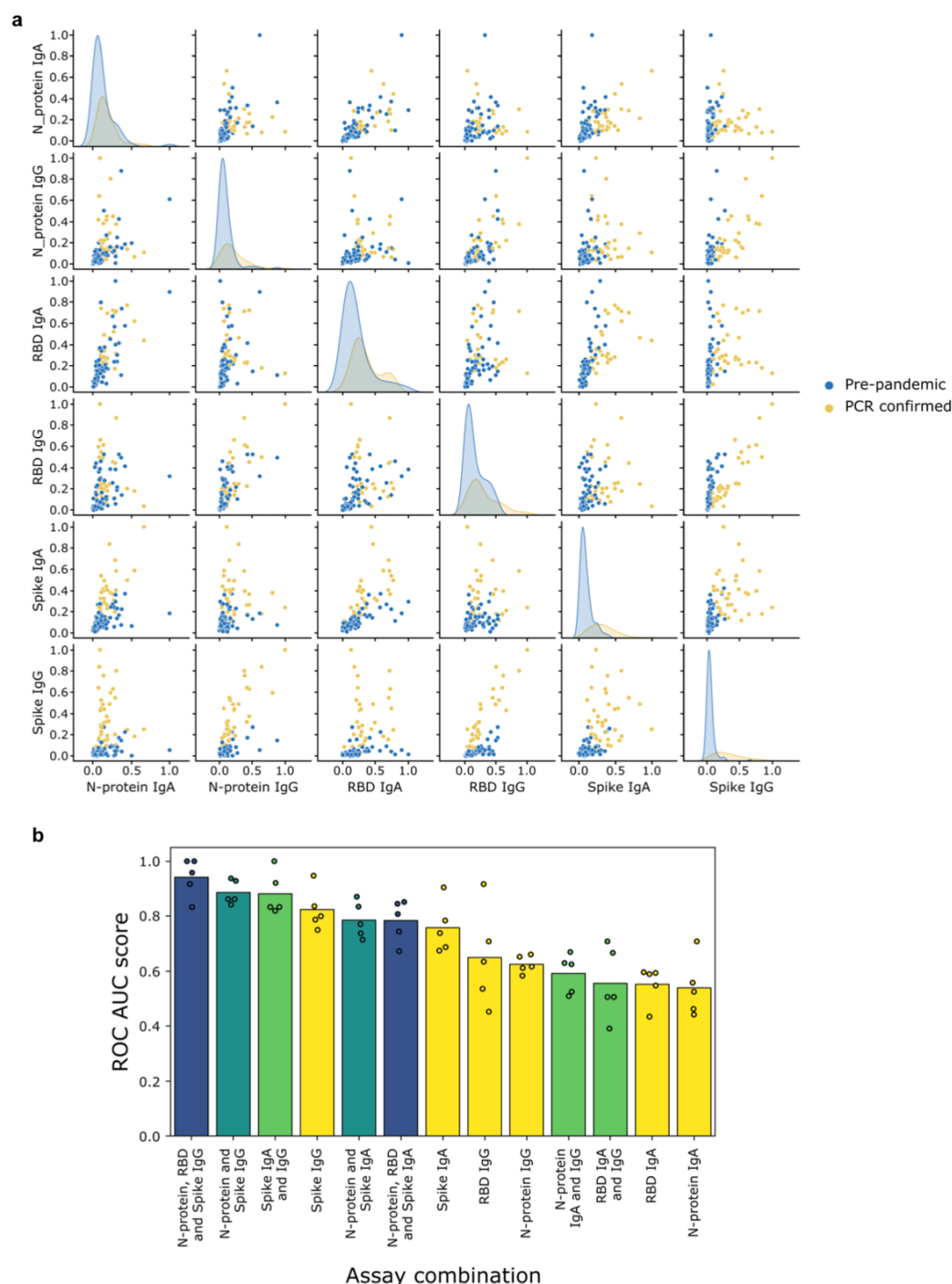
Figure 3: Combining assays improves discriminatory performance. a, Pairwise scatter plots and kernel density estimates of antibody responses for pre-pandemic (blue) and SARS-CoV-2 PCR-confirmed (orange) samples assayed at a single dilution in each of the 6 assays: spike, N-protein, RBD IgA (1 in 10) and IgG (1 in 5). The kernel density estimates along the diagonal represent the distribution of responses measured for a single assay, whilst the scatter plots compare the responses measured across two different assays. b, Comparison of the performance (measured via ROC AUC score) of AdaBoost models trained either with one of the 6 individual assays (yellow bars and dots), or with a selected combination of those assays (green, turquoise, blue bars and dots). The models were trained using 5-fold cross-validation: the dots represent the ROC AUC scores measured for the individual folds, whilst the bars represent the mean of these 5 scores. ROC AUC score = area under the receiver operating characteristic curve.
