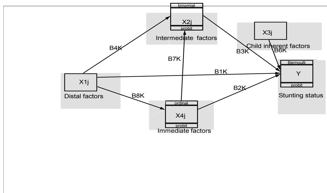
Figure 2: The generalized structural equation model; Note At each level the vector contains either count, discrete, continuous or ordinal data. The family and link descriptions may not carry much sense at this point in time.
