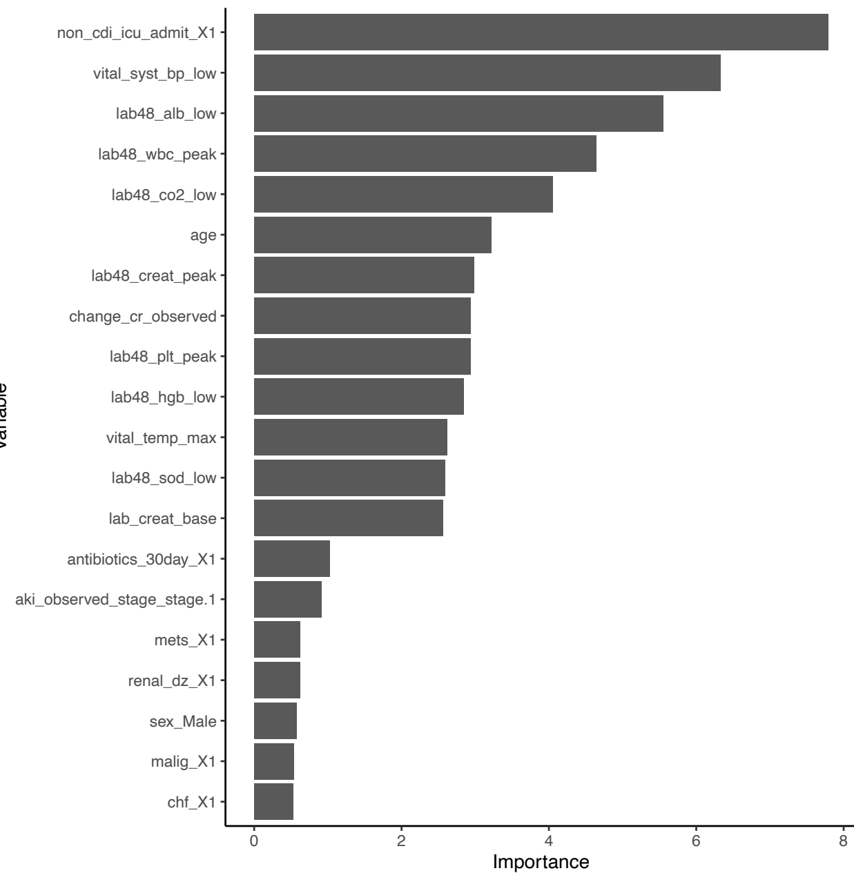
Random Forest Variable Importance Plot
