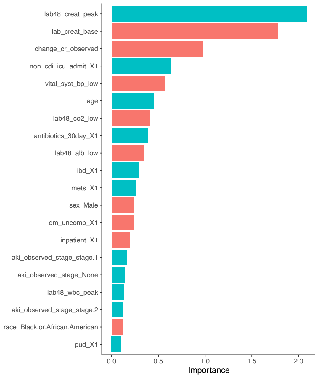
Lasso Variable Importance Plot
