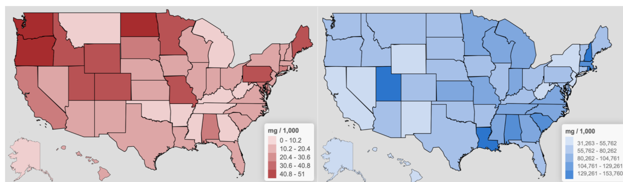
Figure 2. Heat maps of the per capita drug weights of methamphetamine (left) and amphetamine (right) in milligrams per 1,000 people by US state in 2019.
