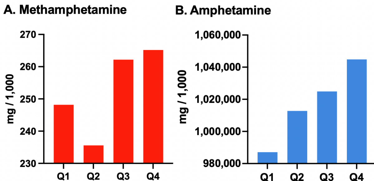
Figure 1. Total per capita quarterly drug distribution of (A) methamphetamine and (B) amphetamine in milligrams per 1,000 people in the US in 2019 as reported to the Drug Enforcement Administration's Automated Reports and Consolidated Orders System. Note restricted Y-axis range to improve viewability.
