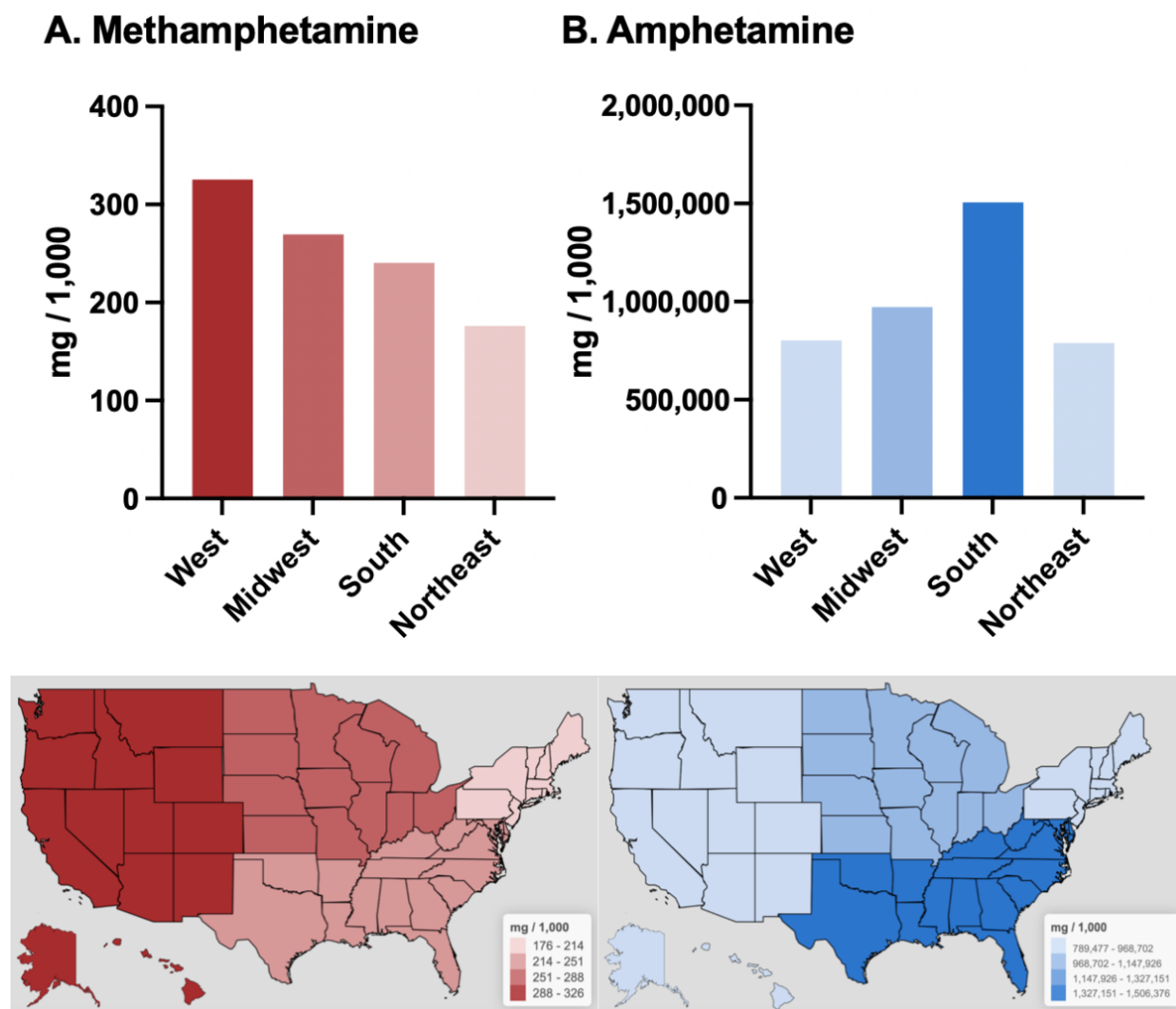
Figure 3. Total per capita drug weights of (A) methamphetamine and (B) amphetamine in milligrams per 1,000 people by region of the US in 2019. Heat maps of the total per capita drug weights of methamphetamine (bottom left) and amphetamine (bottom right) in milligrams per 1,000 people by region of the US in 2019.
