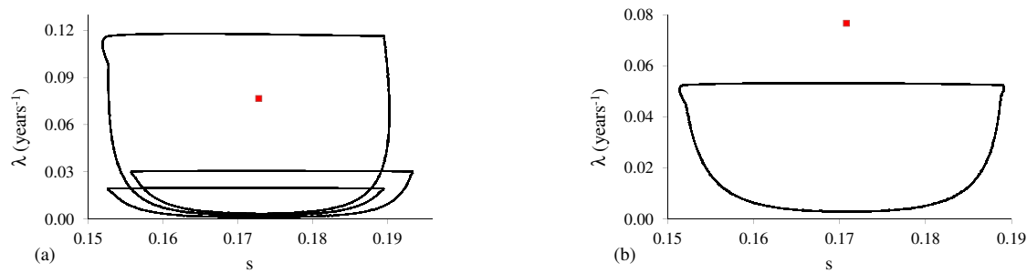
Figure 14: Asymptotic curves for: (a) p = 19.367\% , a three cycles orbit, and (b) p = 19.368\% , a one cycle orbit.
