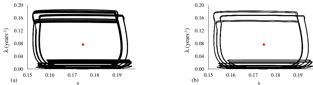
Figure 13: Asymptotic curve for: (a) p = 19.010\% , irregular but a seventy two cycles orbit for decreased relative error \varepsilon , and (b) p = 19.018\% , an eighteen cycles orbit.
