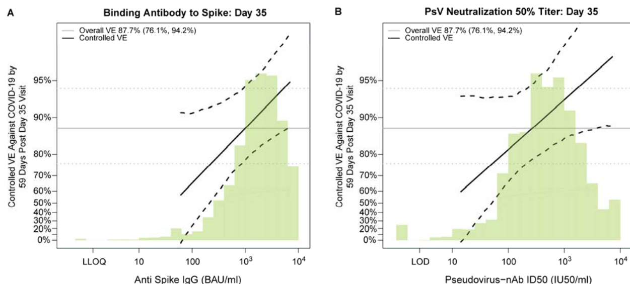
Figure 5. Vaccine efficacy by D35 antibody marker level in baseline SARS-CoV-2 negative per-protocol vaccine recipients (U.S. study sites). Curves shown are for D35 (A) anti-spike IgG concentration or (B) pseudovirus (PsV)-nAb ID50 titer. The dotted black lines indicate bootstrap pointwise 95% confidence intervals. The green histogram is an estimate of the density of D35 antibody marker level and the horizontal gray line is the overall vaccine efficacy from 7 to 59 days post D35, with the dotted gray lines indicating the 95% confidence intervals. Analyses adjusted for baseline risk score. Curves are plotted over the antibody marker range from the 2.5 th percentile to the 97.5 th percentile: 60.9 to 6934 BAU/ml for anti-spike IgG (where 6934 is the ULOQ) and 14.2 to 7230 IU50/ml for PsV-nAb ID50.
