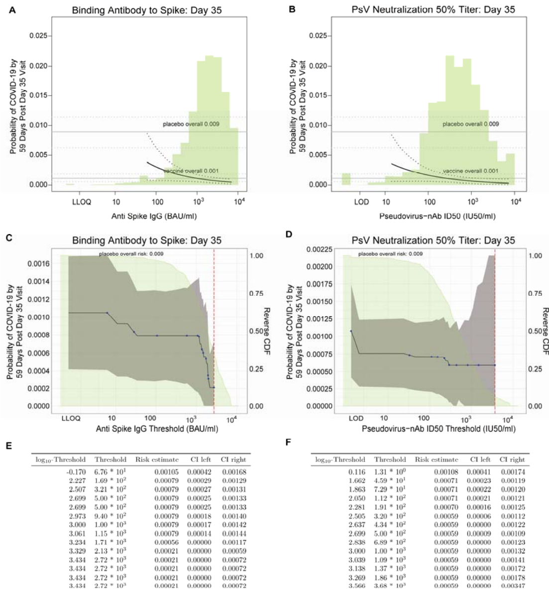
Figure 4. Analyses of D35 antibody markers as a correlate of risk in baseline SARS-CoV-2 negative per-protocol vaccine recipients (US study sites). (A, B) Baseline risk score-adjusted cumulative incidence of COVID-19 by 59 days post D35 by D35 (A) anti-spike IgG or (B) pseudovirus (PsV)-nAb ID50 titer, estimated using a marginalized Cox model. The dotted black lines indicate bootstrap pointwise 95% CIs. The upper and lower horizontal gray lines are the overall cumulative incidence of COVID-19 from 7 to 59 days post D35 in placebo and vaccine recipients, respectively. Curves are plotted over the antibody marker range from the 2.5 th percentile to the 97.5 th percentile: 60.9 to 6934 BAU/ml for spike IgG (where 6934 is the ULOQ) and 14.2 to 7230 IU50/ml for PsV-nAb ID50. (C-F) Baseline risk score-adjusted cumulative incidence of COVID-19 by 59 days post D35 by D35 (C, E) anti-spike IgG or (D, F) PsV-nAb ID50 titer above a threshold. The blue dots are point estimates at each COVID-19 primary endpoint linearly interpolated by solid black lines; the gray shaded area is pointwise 95% confidence intervals (CIs). The estimates and CIs assume a non-increasing threshold-
