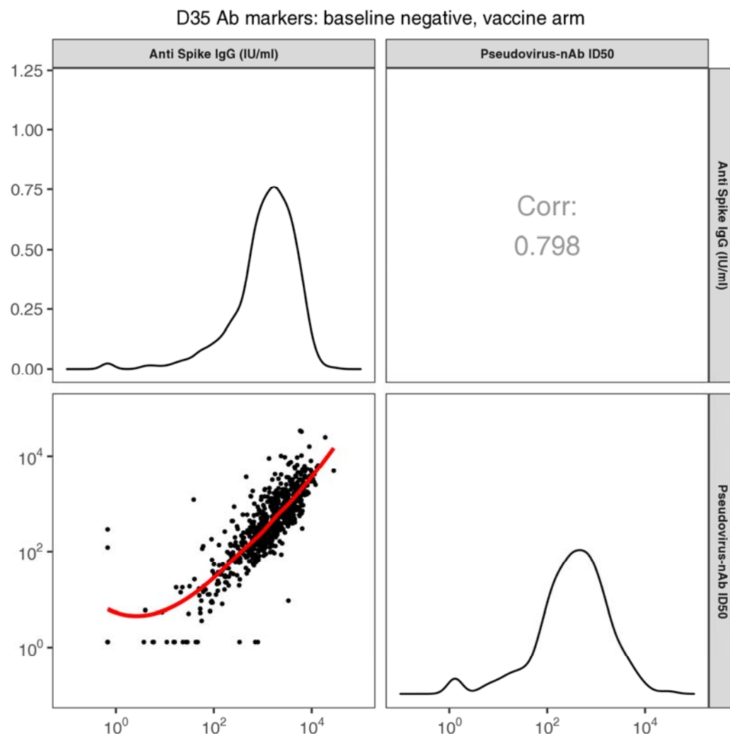
Figure 2. Scatterplot of Day 35 spike IgG vs. pseudovirus (PsV)-nAb ID50 values for baseline SARS-CoV-2 negative per-protocol vaccine recipients in the immunogenicity subcohort (U.S. study sites). Corr, Spearman rank correlation.
