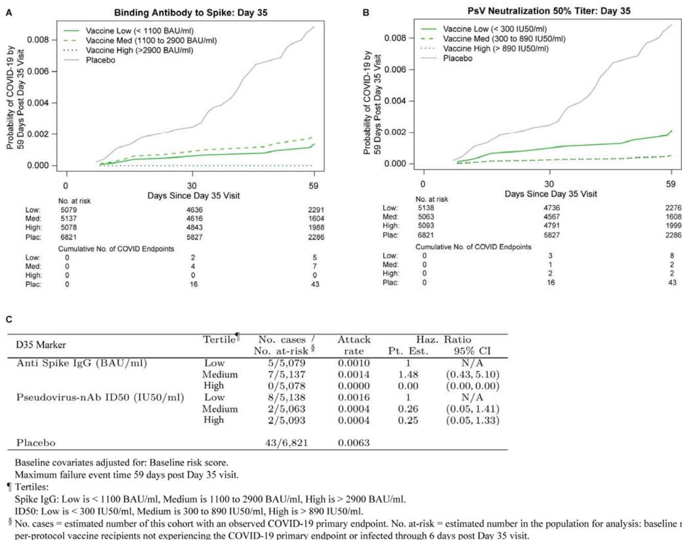
Figure 3. COVID-19 risk by D35 antibody marker level in baseline SARS-CoV-2 negative per-protocol vaccine recipients (U.S. study sites). Baseline risk score-adjusted cumulative incidence of COVID-19 by Low, Medium, High tertile of D35 antibody marker level. (A, C) Anti-spike IgG concentration; (B, C) pseudovirus (PsV) neutralization ID50 titer. No p-values for hypothesis tests are used because of the small number of COVID-19 breakthrough cases, as specified in the Statistical Analysis Plan.
