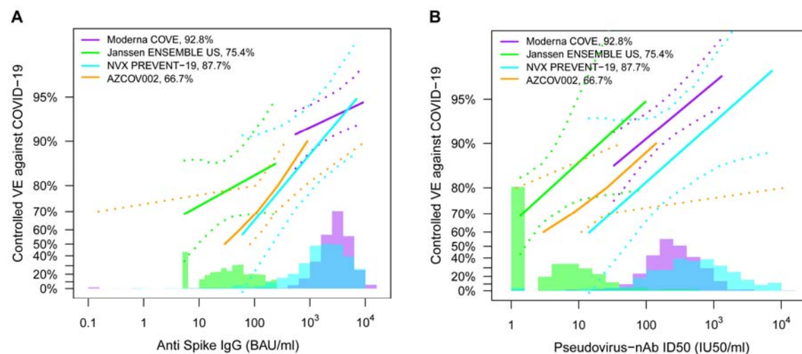
Figure 6. Vaccine efficacy (solid lines) in baseline SARS-CoV-2 negative per-protocol participants by post-vaccination antibody marker level in four randomized, placebo-controlled COVID-19 vaccine efficacy trials. Vaccine efficacy was estimated using the marginalized Cox proportional hazards implementation of Gilbert et al. 42 Vaccine efficacy (VE) estimates are shown by A) anti-spike IgG concentration [D57 in COVE, D29 in ENSEMBLE-United States sites (ENSEMBLE-US), D35 in PREVENT-19, D56 in COV002] or by B) pseudovirus (PsV)-nAb ID50 titer (D57 in COVE, D29 in ENSEMBLE-US, D35 in PREVENT-19, D56 in COV002). The dashed lines indicate bootstrap point-wise 95% confidence intervals. The follow-up periods for the VE assessment were: COVE (doses D1, D29), 7 to 100 days post D57; ENSEMBLE-US (one dose, D1), 1 to 53 days post D29; PREVENT-19 (doses D0, D21), 7 to 59 days post D35; COV002 (doses D0, D28; 28 days post D28 until the end of the study period). The histograms are an estimate of antibody marker density in baseline SARS-CoV-2 negative per-protocol vaccine recipients. Curves are plotted over the following antibody marker ranges: A) COVE: 2.5 th percentile to 97.5 th percentile of marker, ENSEMBLE-US: 2.5 th percentile to 97.5 th percentile, PREVENT-19: 2.5 th percentile to 97.5 th percentile, COV002: 29 to 899 BAU/ml; B) COVE: 10 IU50/ml to 97.5 th percentile of marker, ENSEMBLE-US: 2.5 th percentile to 97.5 th percentile, PREVENT-19: 2.5 th percentile to 97.5 th percentile, COV002: 3 to 140 IU50/ml. Baseline covariates adjusted for were: COVE: baseline risk score, comorbidity status, and Community of color status; ENSEMBLE-US, baseline risk score; PREVENT-19: baseline risk score; COV002: baseline risk score.
