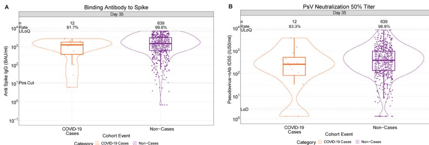
Figure 1. D35 antibody marker level by COVID-19 outcome status in baseline SARS-CoV-2 negative per-protocol vaccine recipients (U.S. study sites). (A) Anti-spike IgG
