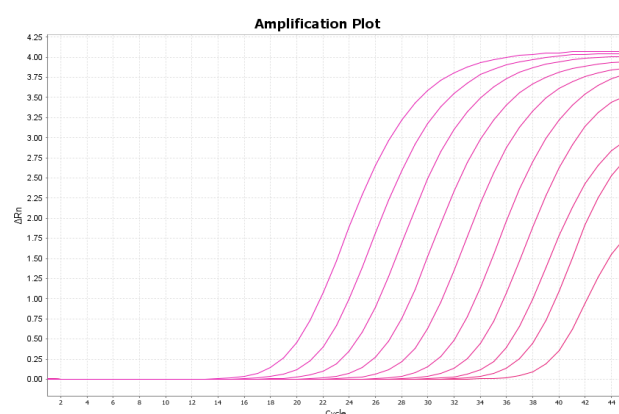
Figure 4. \Delta R_n vs cycle representation of the qPCR performed on the QuantStudio™ 7 Flex Real-Time PCR System. MPXV PCR amplification curves from successive 5-fold serial dilutions of a positive sample with Ct values ranging from 16.5 to 37.3.
