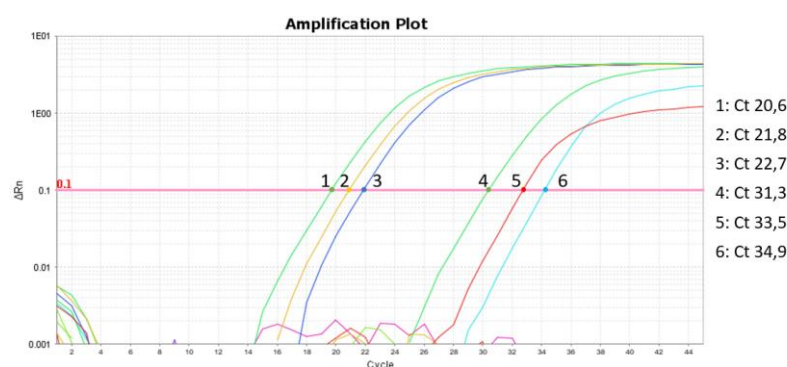
Figure 5. \Delta R_n vs cycle representation of the qPCR performed on the QuantStudio™ 7 Flex Real-Time PCR System. PCR amplification curves of DNA samples from the ongoing human MPXV-outbreak, which started in May 2022. 1: Positive control, 2-6: Clinical DNA samples.
