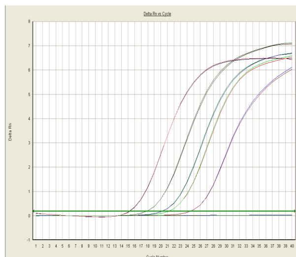
Figure 2. \Delta Rn vs cycle representation of the real-time PCR performed on an AB™ 7500 Fast Real-Time PCR system. Data were obtained using the 7500 Fast System Software v1.3.1 with primers and hybridization probe calculated for MPXV. The detection signal of 6-FAM dye conjugated with MPXV-probe is 518 nm.
