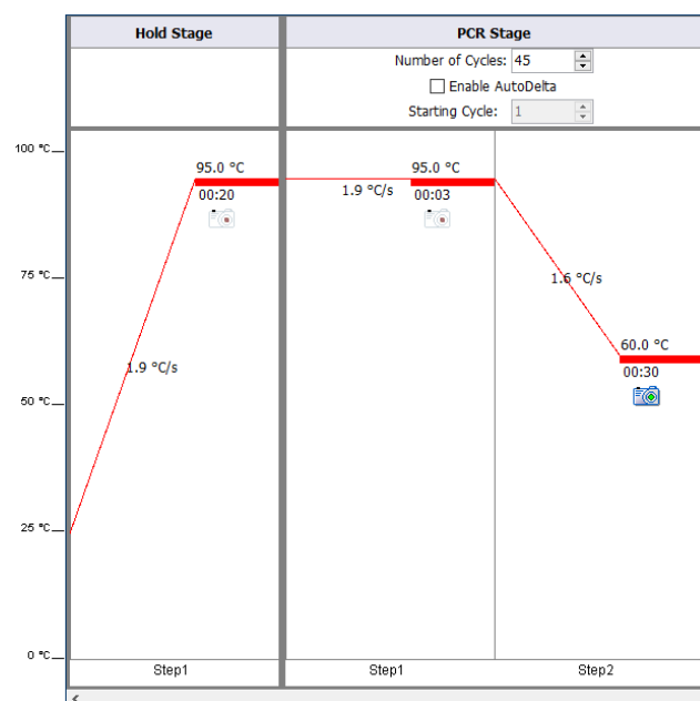
Figure 1. PCR conditions for MPXV diagnosis on QuantStudio™ 7 Flex RT PCR System
