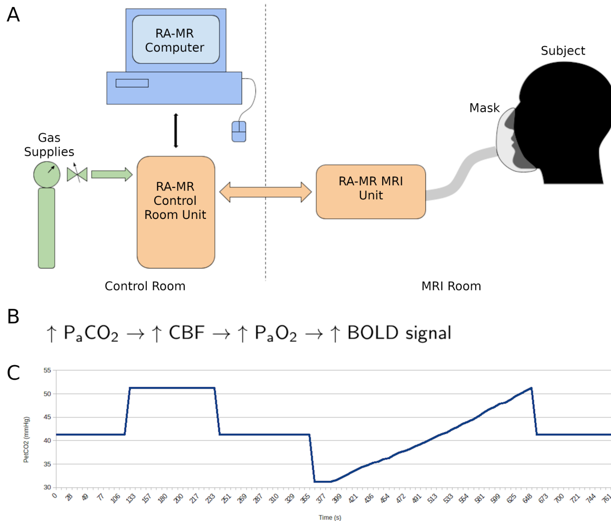
Figure 1: Respiract (RA-MR™) and Cerebrovascular Reactivity (CVR) Schematic Diagram. A) Provides a diagram of the basic components of the RA-MR system. The participant is breathing through a mask that has gas being detected and administered by the RA-MR MRI Unit. This unit in turn receives gas from the RA-MR Control Room Unit, which is connected directly to the gas supplies and the RA-MR Computer. B) The basic sequence of events behind hypercapnia and the increase in fMRI signal. C) Target end-tidal PCO_2 ( P_{ET}CO_2 ) schematic over the course of the CVR fMRI scan.
