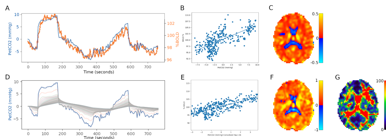
Figure 2: CVR Processing. A) Alignment of P_{ET}CO_2 (blue) with the average BOLD signal (orange). B) Linear least-squares fit of the BOLD response to the P_{ET}CO_2 stimulus on a voxel-by-voxel basis: CVR_{whole} . C) Resulting axial slice of a CVR map (in units \Delta\%BOLD/mmHg ). D) Set of curves resulting from the convolution of P_{ET}CO_2 . E) The regression with the best fit between the convolved P_{ET}CO_2 and the BOLD signal: ssCVR. F) Resulting axial slice of a ssCVR map. G) Resulting axial slice of a tau map.
