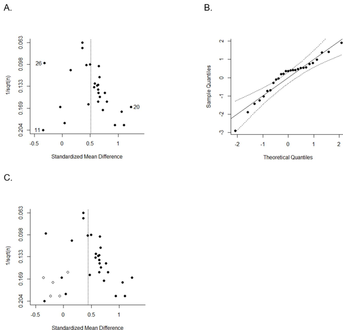
Figure 3: Plots for assessment of publication bias. (A) Funnel plot for SSRT plotting SMDs against the inverse of the square root of the sample size. (B) Normal quantile-quantile plot, plotting the quantiles of a standard normal distribution against the quantiles of the observed distribution. The points should fall on a straight line and inside the 95%-confidence bands. (C) Funnel plot for SSRT plotting SMDs against the inverse of the square root of the sample size adjusted for publication bias using the trim-and-fill method (filled dots: observed effect estimates, non-filled dots: imputed effect estimates). 11 Cubillo et al. (2010), 20 Murphy et al. (2002), 26 Szekely et al. (2017).
