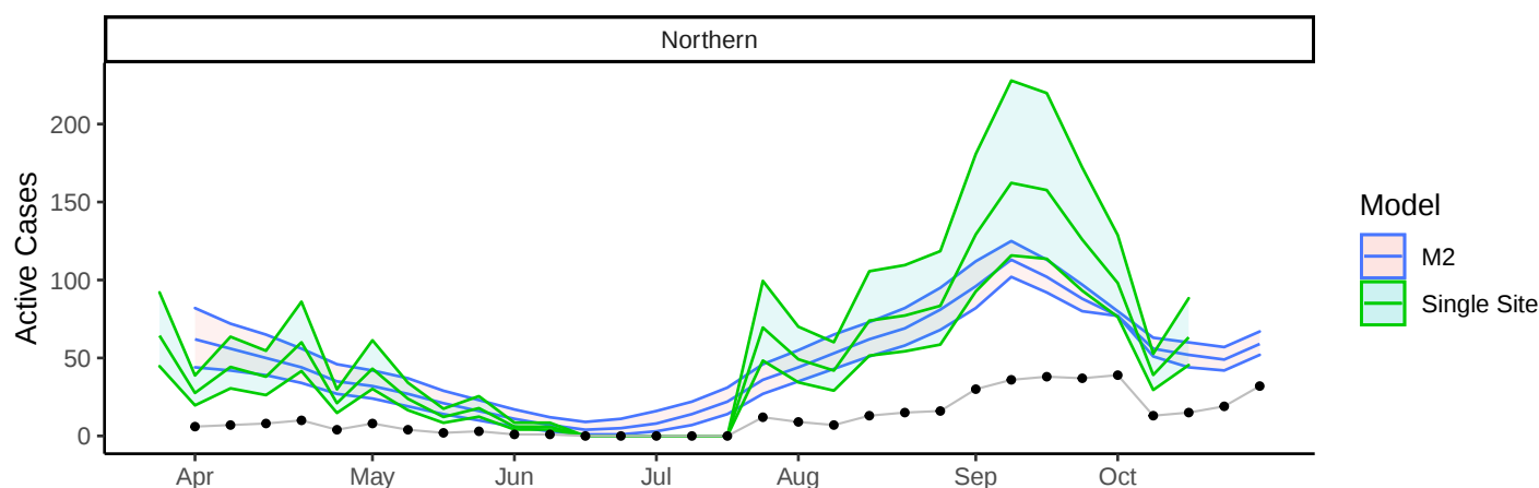
Figure 7: Plot of active cases for the Northern Health Authority region. Data starts on 2 Apr 2020 (Week 1) and ends on 30 Oct 2020 (Week 31). The blue band shows the 95% credible interval for total active cases as estimated using model M2. The green bands show the 95% confidence intervals for total active cases as estimated using the single site model from Parker et al. (2021), denoted Single Site. The black dotted line shows the newly detected active cases each week.
