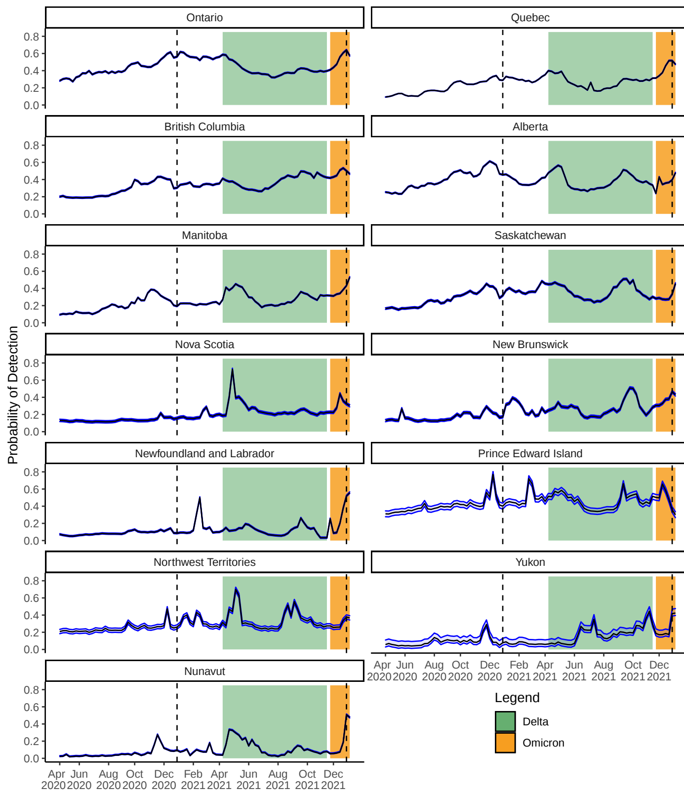
Figure 3: Estimated weekly detection probability (blue) for active COVID-19 cases for each province or territory from 23 Apr 2020 to 6 Jan 2022. The time periods for the two variants of concern—Delta and Omicron—are depicted with coloured bands. The two vertical dashed lines indicate 1 Jan 2021 and 1 Jan 2022. Bands show 95% credible intervals.
