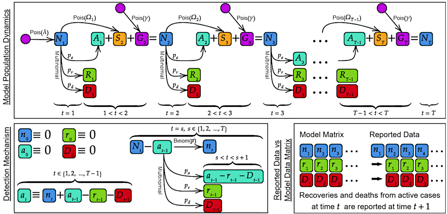
Figure 1: Diagram of single-site model. Top: The disease dynamics and state process. Bottom left: The detection mechanisms. Bottom right: Data reporting times.
