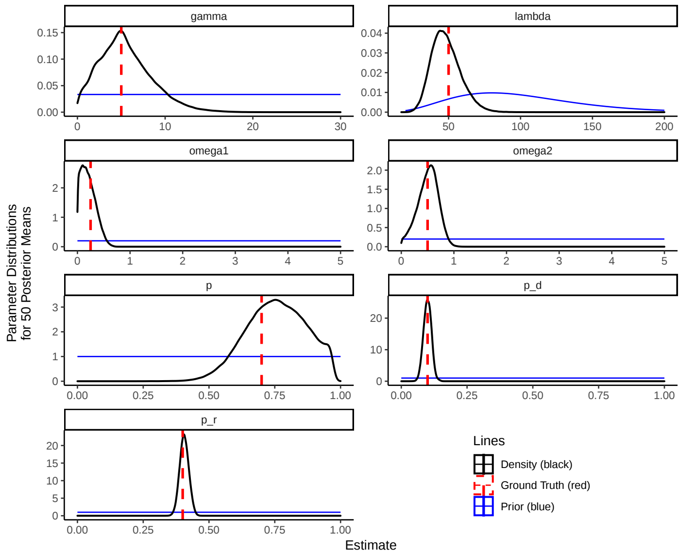
Figure S8: Density plots showing posterior means for each estimated parameter. Fifty simulation runs were used. Red dashed lines indicate the ground truth parameter values for the simulation. Posterior modes are close to ground truth parameter values.
