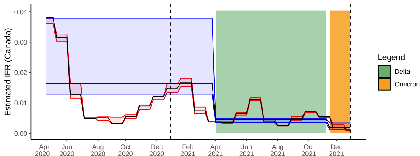
Figure 5: Estimated infection fatality rate (IFR) for COVID-19 infections within Canada. The time periods for the two variants of concern Delta and Omicron are depicted with coloured bands. The estimated IFR for each time period is 0.015 (early pandemic period), 0.005 (Delta period), and 0.002 (Omicron period). The two vertical dashed lines indicate 1 Jan 2021 and 1 Jan 2022. Bands show 95% credible intervals. The red shows monthly estimates, while the blue shows estimates for each of the three time periods.
