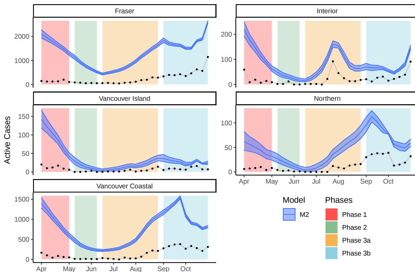
Figure 6: Plots of active cases split by Health Authority Region. Data starts on 2 Apr 2020 (Week 1) and ends on 30 Oct 2020 (Week 31). The blue bands show the 95% credible intervals for total active cases as estimated using model M2. The black dotted line shows the newly detected active cases each week.
