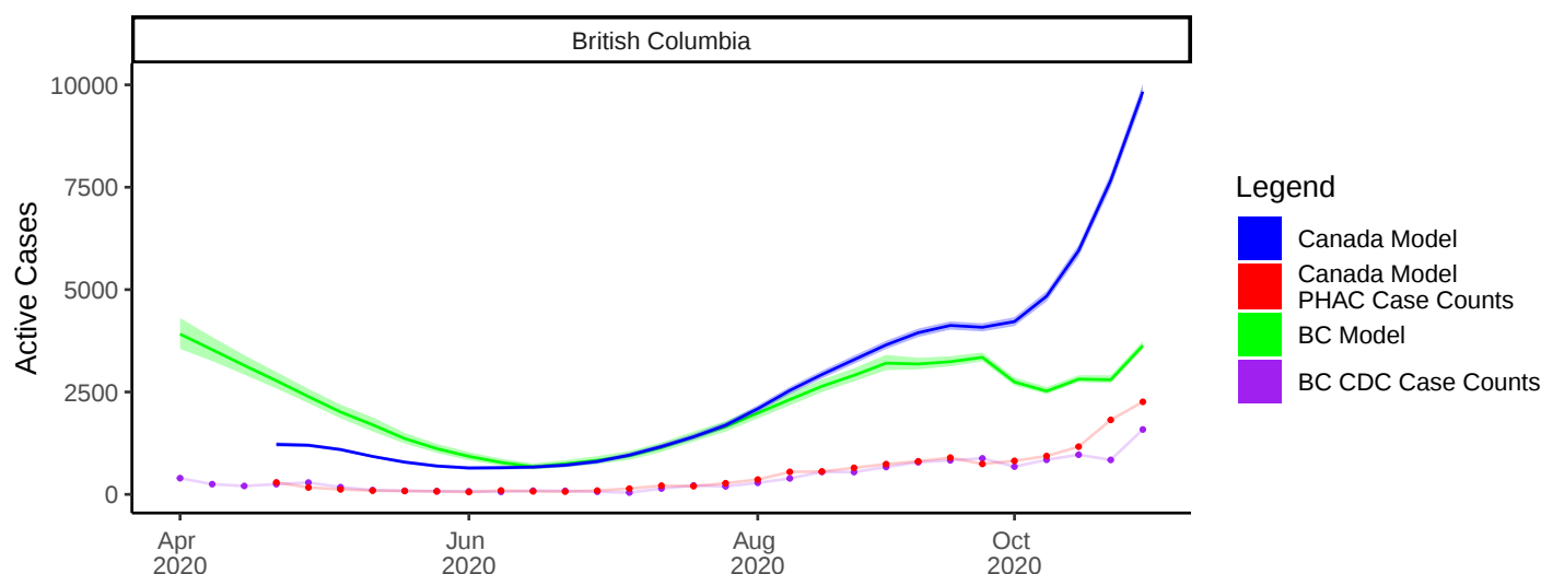
Figure S17: Plots of total active cases for B.C. Data starts on 2 Apr 2020 (Week 1) and ends on 30 Oct 2020 (Week 31). Note that the Canada model data starts on date 23 Apr 2020 (Week 4 of the B.C. only model). The blue bands show the 95% credible intervals for total active cases. Results from the B.C. Health Authority case study, summed over regions, are shown in green, with data shown in purple. Results from the Canada case study, subset to B.C. and Weeks 1 to 31, are shown in blue, with data shown in red. The black dotted line shows the newly observed active cases each week.
