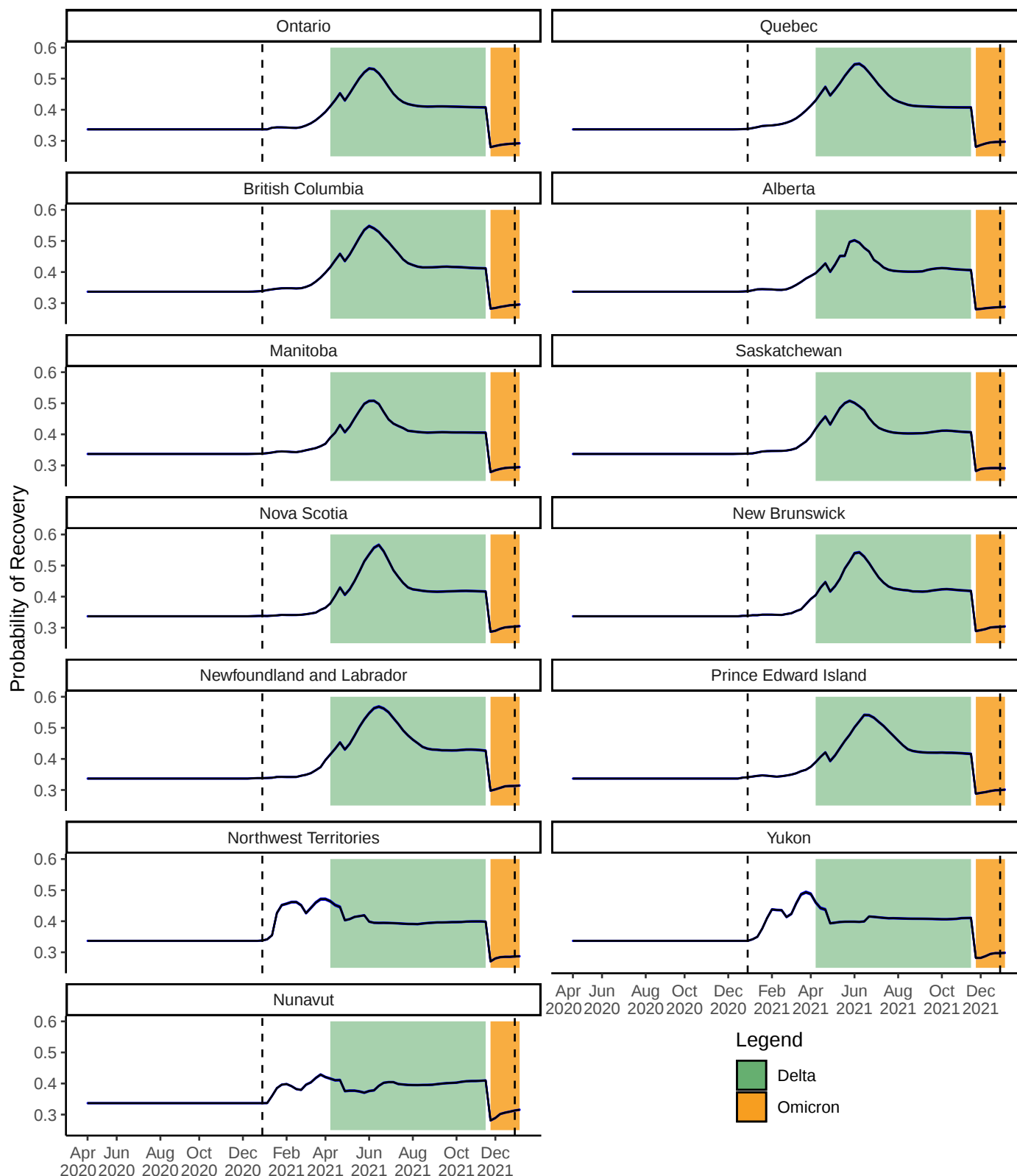
Figure S13: Estimated weekly probability of recovery (blue) for active COVID-19 cases for each province/territory from 2 Apr 2020 to 6 Jan 2022. The time periods for the two variants of concern Delta and Omicron are depicted with coloured bands, indicating the first observations in Canada. The two vertical dashed lines indicate 1 Jan 2021 and 1 Jan 2022. Bands show 95% credible intervals.
