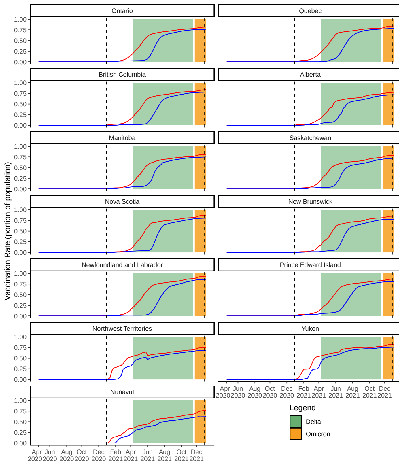
Figure S11: Vaccination rate for each province/territory from 2 Apr 2020 to 6 Jan 2022. The red line indicates at least 1 vaccination dose. The blue line indicates 2 doses. A vaccination rate of 0.5 indicates 50% of the population is vaccinated. The time periods for the two variants of concern Delta and Omicron are depicted with coloured bands, indicating the first observations in Canada. The two vertical dashed lines indicate 1 Jan 2021 and 1 Jan 2022.
