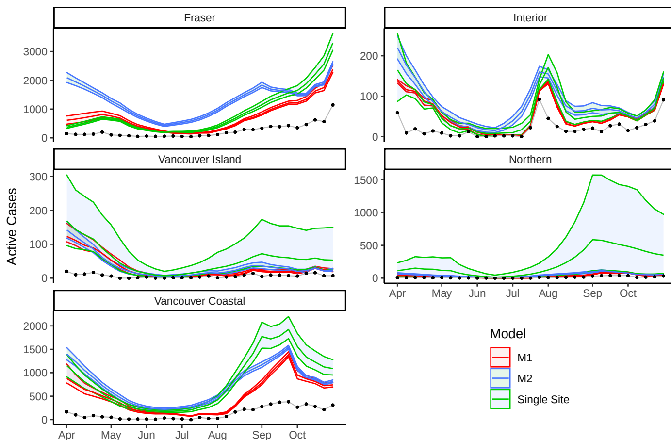
Figure S16: Plots of active cases split by Health Authority Region of B.C. Data starts on 2 Apr 2020 (Week 1) and ends on 30 Oct 2020 (Week 31). The red bands show the 95% credible intervals for total active cases as estimated using model M1, the best fitted model according to WAIC. The blue bands show the 95% credible intervals for total active cases as estimated using model M2, the second best fitted model according to WAIC. The green bands show the 95% credible intervals for total active cases as estimated using the single site models with testing volume as a covariate for detection probability. The black dotted line shows the newly observed active cases each week (according to data).
