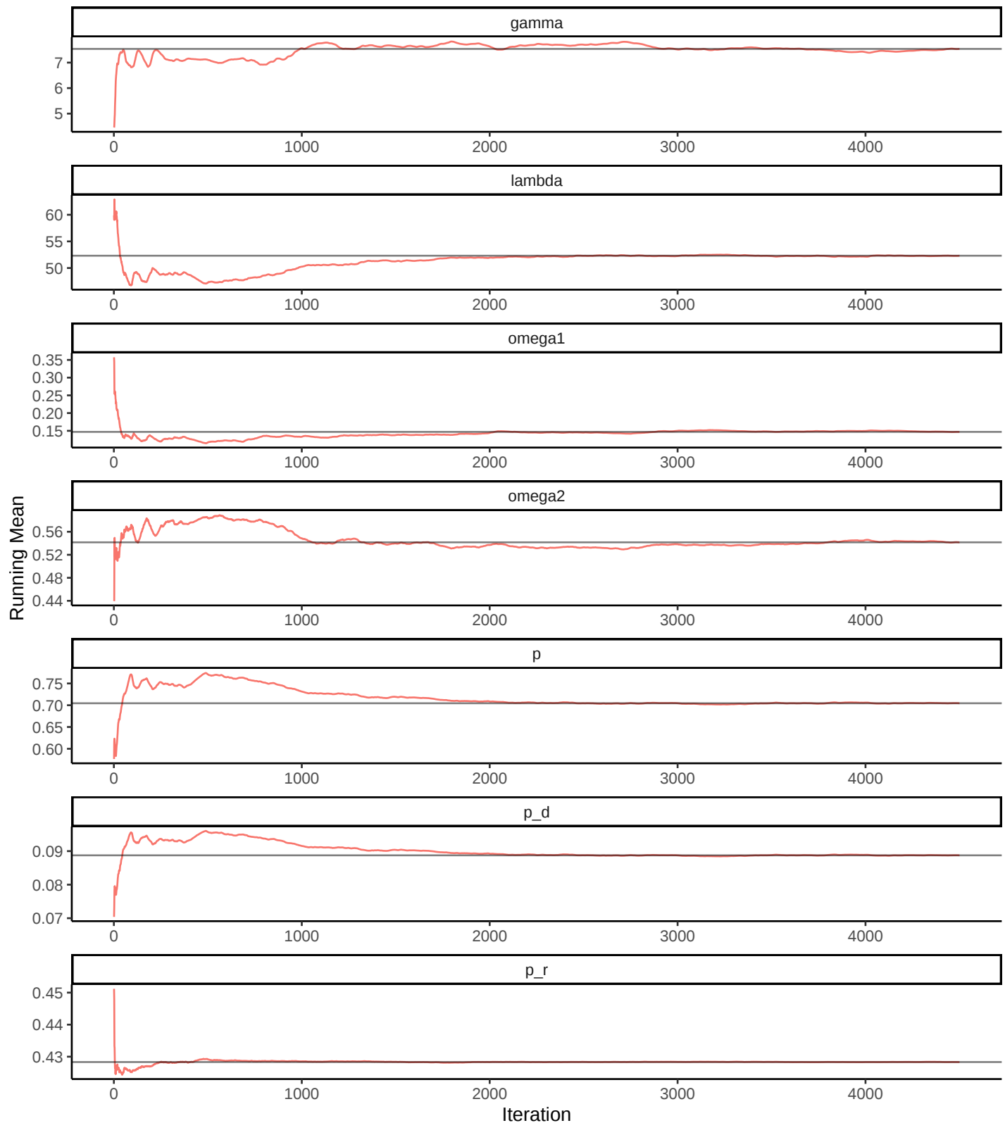
Figure S9: Posterior running means for each estimated parameter for a single fixed replicate (dataset 25 out of 50) of the simulation study. The black horizontal lines indicate the overall mean. Red lines indicate the running means. Running means approach overall means.
