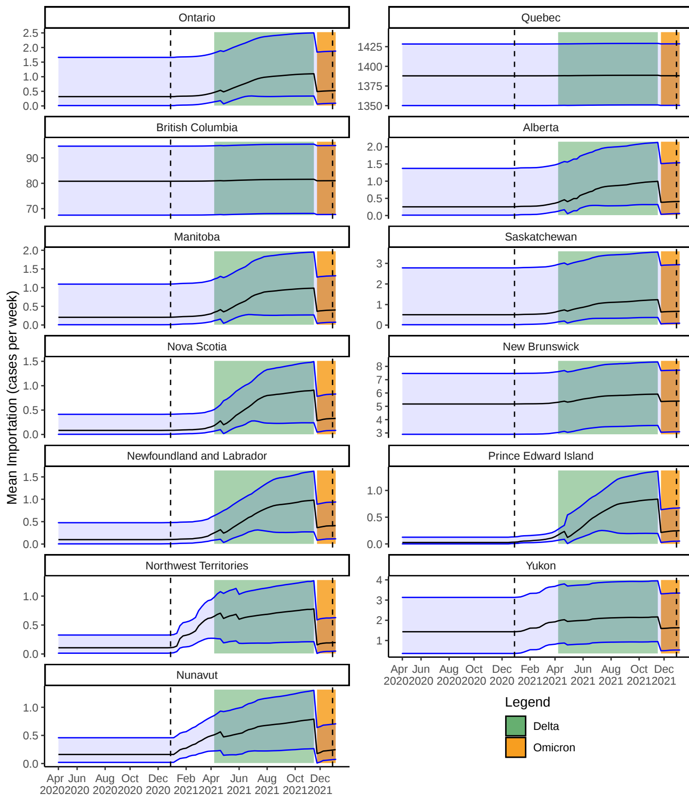
Figure S14: Estimated weekly importation of active COVID-19 cases for each province/territory from 2 Apr 2020 to 6 Jan 2022. The time periods for the two variants of concern Delta and Omicron are depicted with coloured bands, indicating the first observations in Canada. The two vertical dashed lines indicate 1 Jan 2021 and 1 Jan 2022. Bands show 95% credible intervals.
