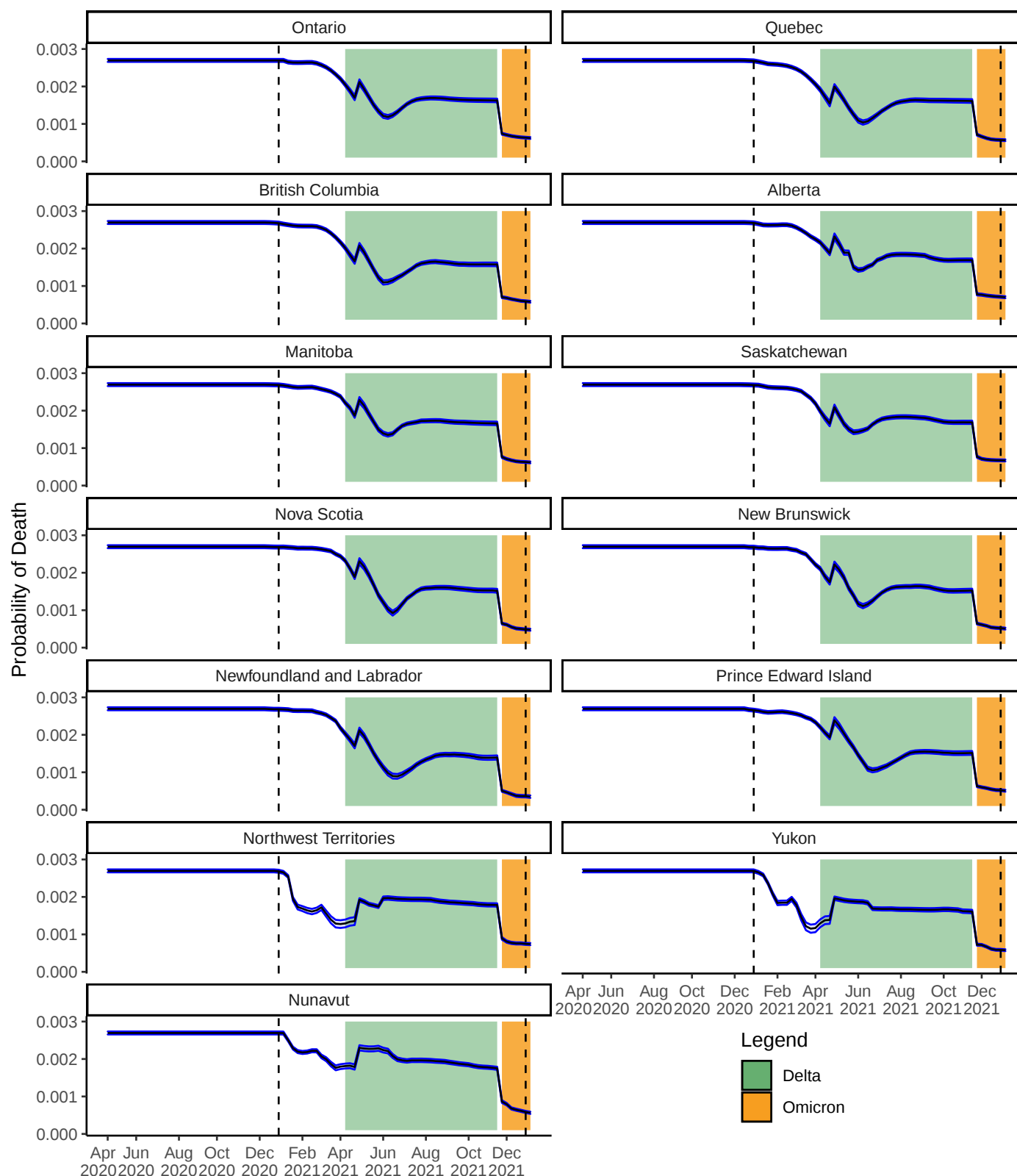
Figure S12: Estimated weekly probability of death (blue) for active COVID-19 cases for each province/territory from 2 Apr 2020 to 6 Jan 2022. The time periods for the two variants of concern Delta and Omicron are depicted with coloured bands, indicating the first observations in Canada. The two vertical dashed lines indicate 1 Jan 2021 and 1 Jan 2022. Bands show 95% credible intervals.
