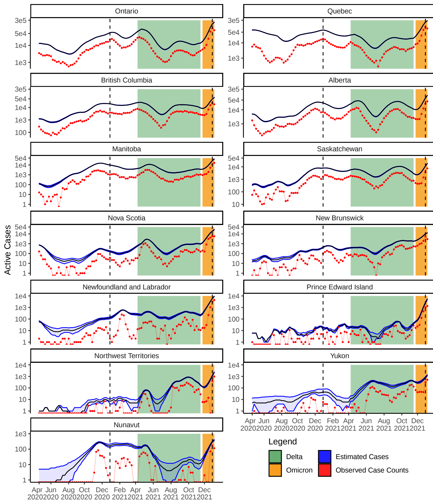
Figure 2: Detected case counts (red) and estimated total active cases (blue) for each province/territory from 23 Apr 2020 to 6 Jan 2022. The time periods for the two variants of concern Delta and Omicron are depicted with coloured bands. The two vertical dashed lines indicate 1 Jan 2021 and 1 Jan 2022. Active cases are plotted on a log scale. Bands indicate 95% credible intervals.
