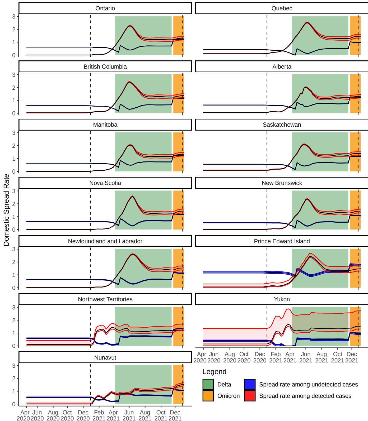
Figure 4: Estimated weekly domestic spread rates for detected (red, \hat{\omega}_2 ) and undetected (blue, \hat{\omega}_1 ) active COVID-19 cases for each province/territory from 23 Apr 2020 to 6 Jan 2022. The time periods for the two variants of concern Delta and Omicron are depicted with coloured bands. The two vertical dashed lines indicate 1 Jan 2021 and 1 Jan 2022. Bands show 95% credible intervals.
