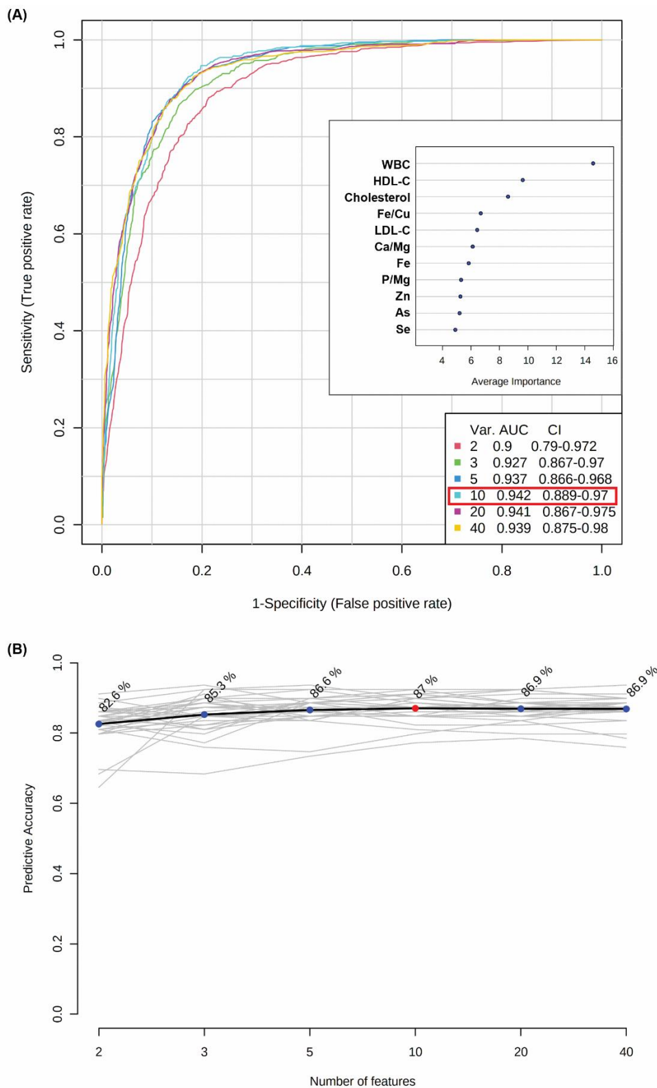
Figure 3. Classification performance of random forest models built with metallomic features and traditional cardiovascular risk factors as shown by (A) ROC curves and most important variables identified in the model, and (B) predictive accuracies.
