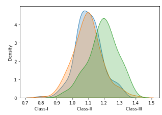
Figure 11. Density plot.
