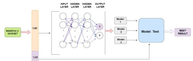
Figure 5. Deep learning model used.
