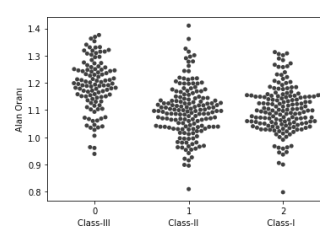
Figure 10. Scatter plot.
