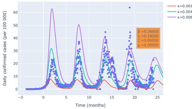
FIG. 4. (a) Comparison of the results of the SBIGR model [Eqs. (14)] with data of newly reported cases for South Africa. Results for different values of \kappa are shown for a fixed value of \kappa/\zeta .
