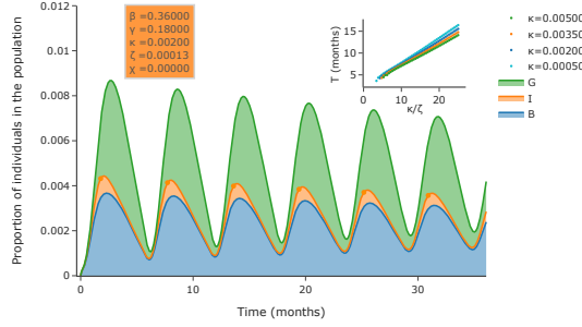
FIG. 3. (a) Numerical integration of the SBIGR model [Eqs. (14)]. The figure shows a stackplot of the quantities B, I, G . Slowly decaying oscillations are observed for this set of parameters. In the inset it is illustrated that the time-interval T between two peaks of the number of infected individuals (indicated by dots in the main plot) is set by the parameter \kappa/\zeta .
