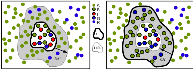
FIG. 2. Graphical representation of the evolution of an (a) acceleration, or (b) deceleration epidemic. The "blob" around the infected I represents all people that are in close contact with contagious individuals. The blob expands when the local concentration of I is large. The blob will shrink if little infected are present. S and B are susceptibles, G, R are removed/recovered. Change in surface, \delta A during a time-interval is indicated as a shaded area.
