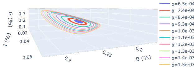
FIG. 5. Phase-space plot of the SBIGR model [Eqs. (14)] with decrease of immunity, \chi > 0 . For the current parameters, the value \chi > 0.0007 , corresponding to a typical immunity decrease time t_{1/2} \approx 1000\text{days} leads to a limit cycle, representing a non-vanishing periodic epidemic. For \chi < 0.0007 , the amplitude of the peaks decreases in time.
