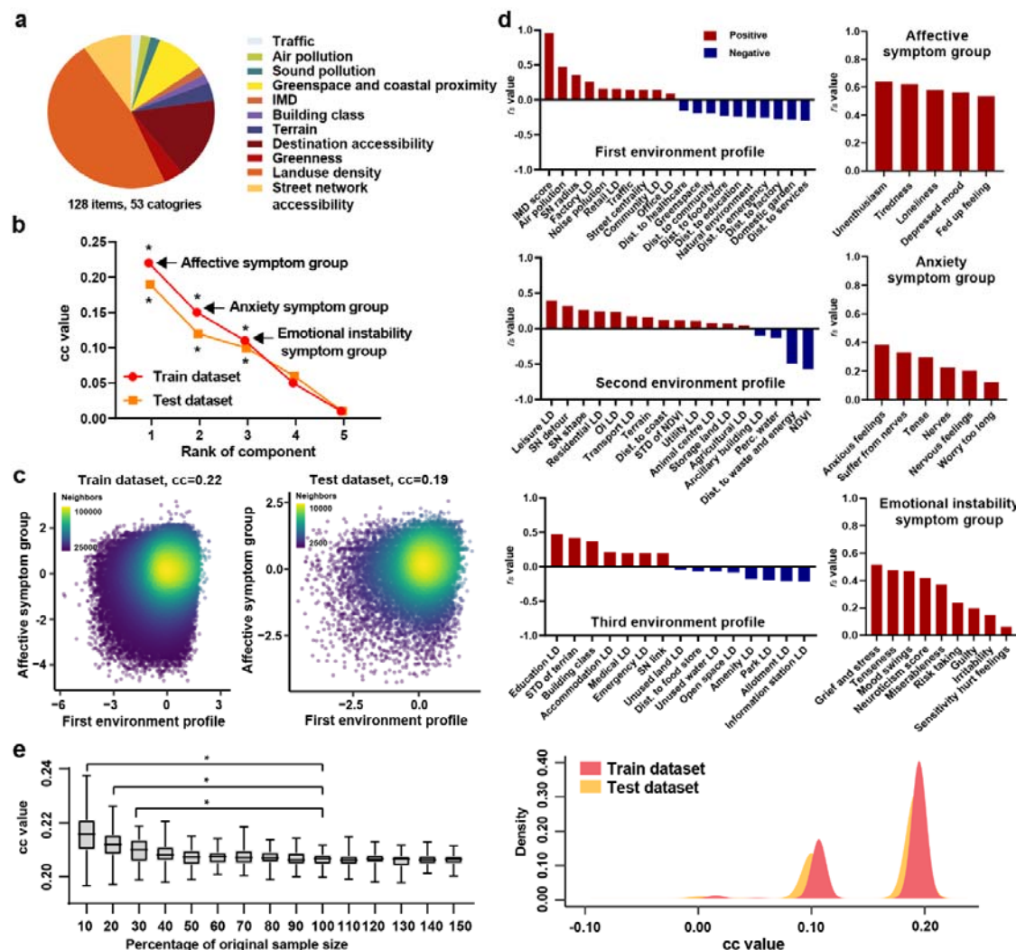
278 Figure 2. Multivariate relation between urban living environment profile and 279 symptoms of mental illness. a. A total of 128 items corresponding to 53 categories of 280 urban living environment are included; b. The sCCA-regression model linking urban 281 living environment to symptoms of mental illness identified three significant correlates 282 in train datasets (red dot), including affective symptoms group ( r=0.22 , 283 P_{\text{permutation}} < 0.001 ), anxiety symptoms group ( r=0.15 , P_{\text{permutation}} < 0.001 ) and emotional
