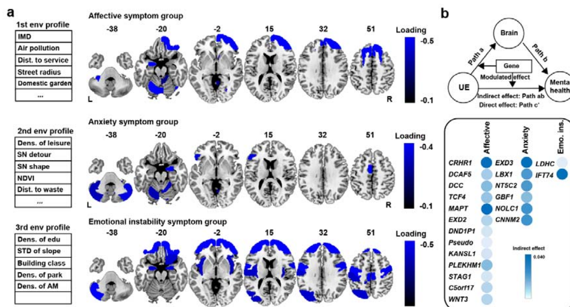
Figure 4. Three-way msCCA regression between urban living environmental profile, regional brain volume and mental illness symptom group, and moderated mediation
