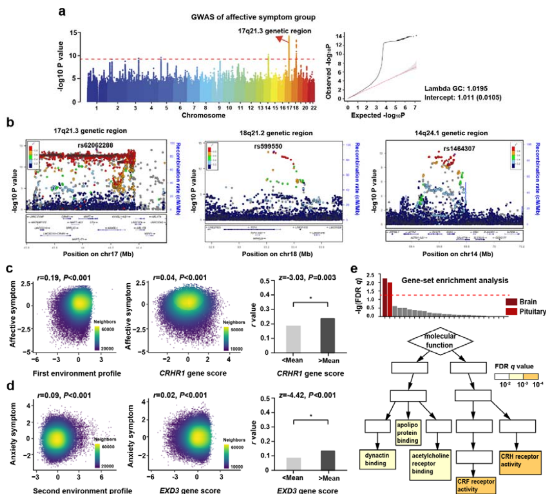
Figure 3. Associations of genomics, urban living environment profiles and mental health symptoms. a. Left. Manhattan plot of GWAS analysis. GWAS of the affective symptom group identifies 2,983 significantly associated SNPs. The strongest association with the affective symptom group was found in a genomic region of chromosome 17q21.3 spanning from position 43487217 to 44862162 (hg19) containing a potential supergene that encodes several genes previously implicated in mental illness. An intron variant rs62062288 located in MAPT gene of chromosome 17 ( P=6.09 \times 10^{-15} ) was the lead SNP; Right. Quantile-quantile plot of GWAS analysis.
