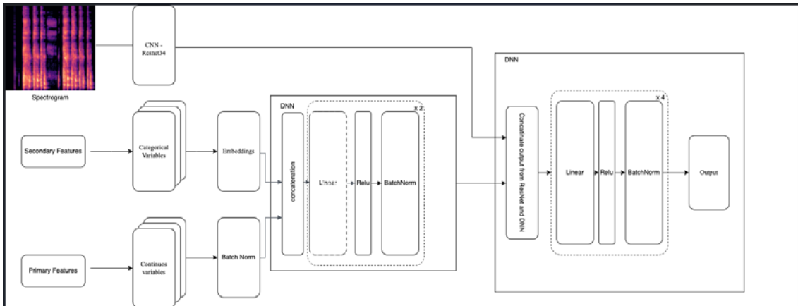
Figure 2: Illustration of the combined logic - combining Feedforward Artificial Neural Network (FFANN) model and Convolutional Neural Network (CNN) outputs
