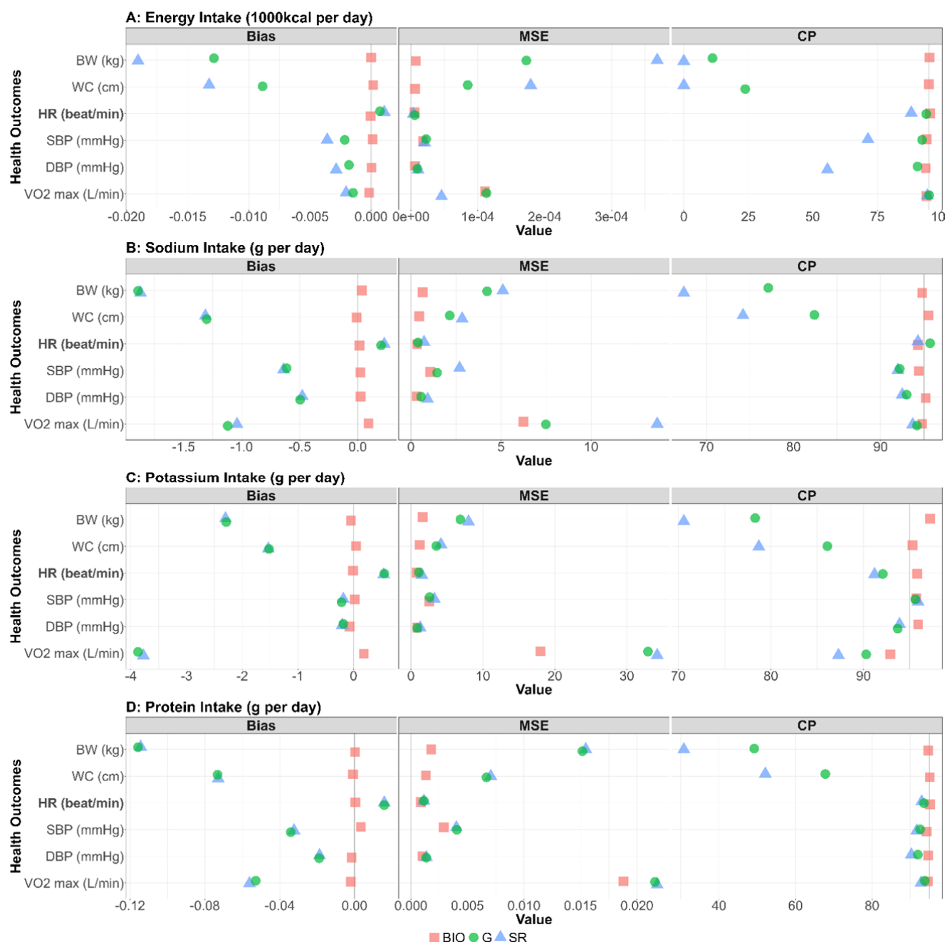
Figure 3: Bias, MSE, and coverage probability in the simulation study
