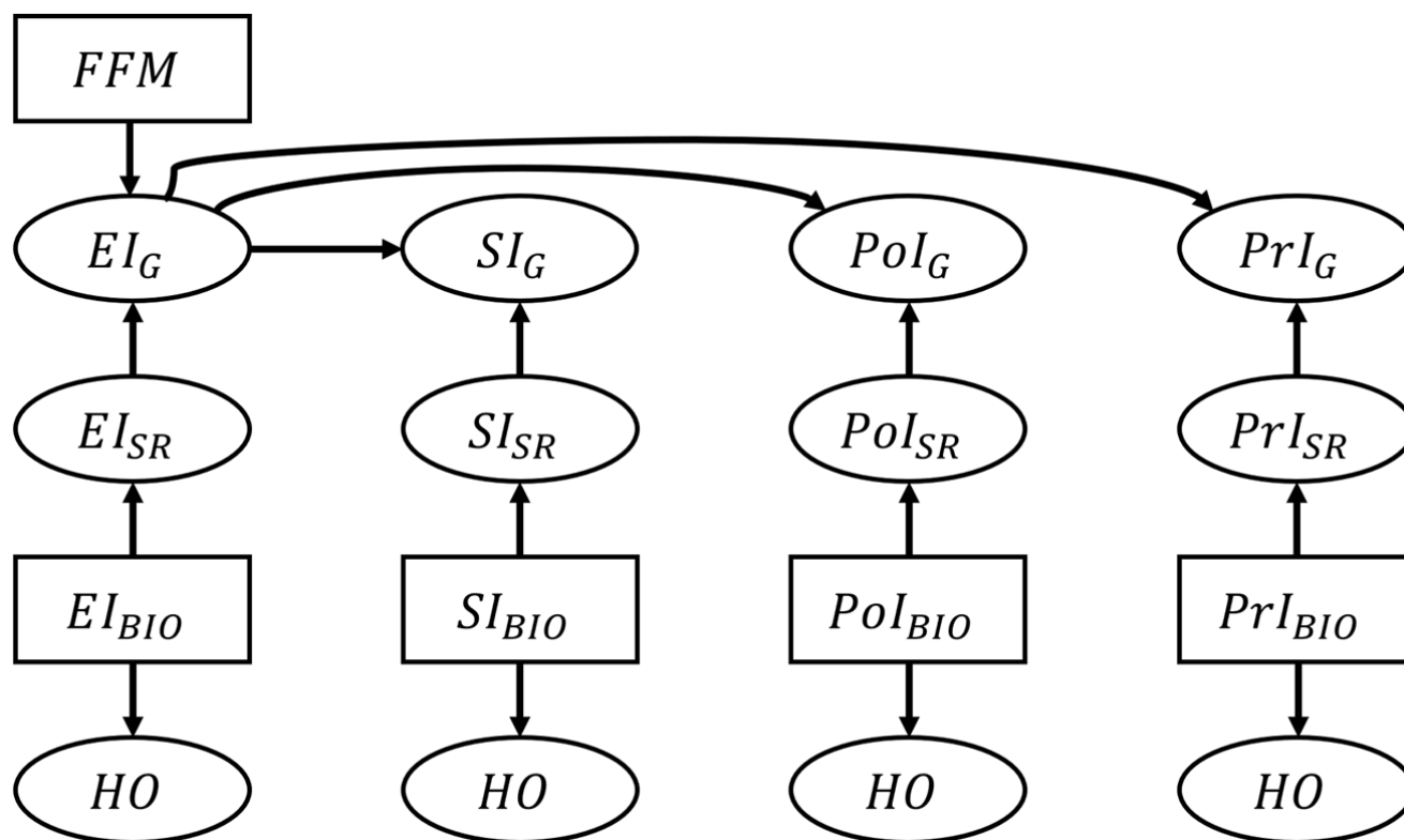
Figure 4: Schematic illustration of the data generation process for the nutrition intake and health outcomes
