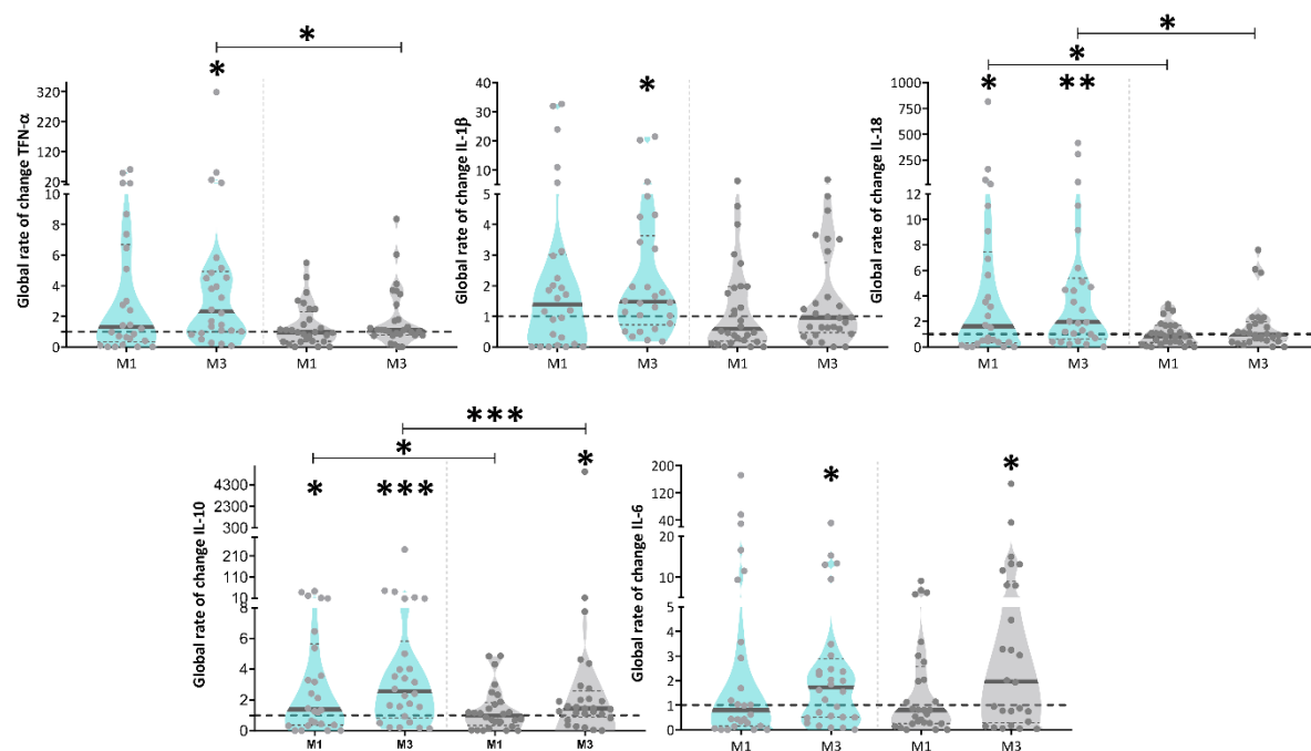
Figure 2. The inflammatory profile of people with COPD changes upon pulmonary rehabilitation. Global rate of change represents the ratio between cytokine values measured at baseline and M1 or M3 ( i.e. M1/M0 and M3/M0). Differences between M1 and the baseline and between M3 and the baseline were assessed by Wilcoxon signed-rank, in each group (intervention (blue) and control (grey)). Differences between groups at M1 and M3 were assessed by Mann-Whitney U-test. p < 0.05 , **p < 0.01 , ***p < 0.001 . All cytokines for which a significant shift was observed are represented in this figure. Supplementary figure 2 shows the data for the remaining 8 cytokines.
