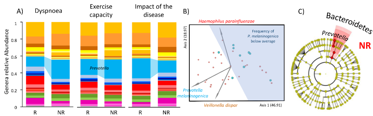
Figure 3. Responders and non-responders present distinct microbiota profiles prior to pulmonary rehabilitation. A) Mean frequency of phyla and genera of bacteria present in Responders (R) and non-responders (NR) to dyspnoea, exercise capacity and impact of the disease. B) R and NR to dyspnoea showed distinct microbiota composition prior to PR (PERMANOVA, p=0.04 ). PCoA analysis using Emperor on Weighted UniFrac distance. The biplot (grey arrows) represent the 3 most relevant ASVs for R and NR segregation. Prevotella melaninogenica (ASV: d0b698c7298bf04110a6d2f220879bfb) was the major contributor for segregation of R and NR followed by Veillonella dispar (ASV: 5608c3e6c9de9ceb79610e7786bd0ac) and Haemophilus parainfluenzae (ASV: e27680d4009f98f30248d823bc17fb8e). In blue is represented the area where samples presented a mean frequency of P. melaninogenica below the average of the dataset. 78% of R showed reduced mean frequencies of P. melaninogenica prior to PR while only 37% of NR followed the same trend. C) Cladogram highlighting differentially abundant genera between R and NR to dyspnoea prior to PR, inferred by linear discriminant analysis (LEfSe) at a significance cut-off of 3. Prevotella is significantly enriched in NR to dyspnoea, with an effect-size of 9.
