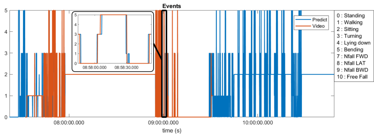
Fig 2. Predicted activities compared to the video annotations obtained from a patient at home environment
