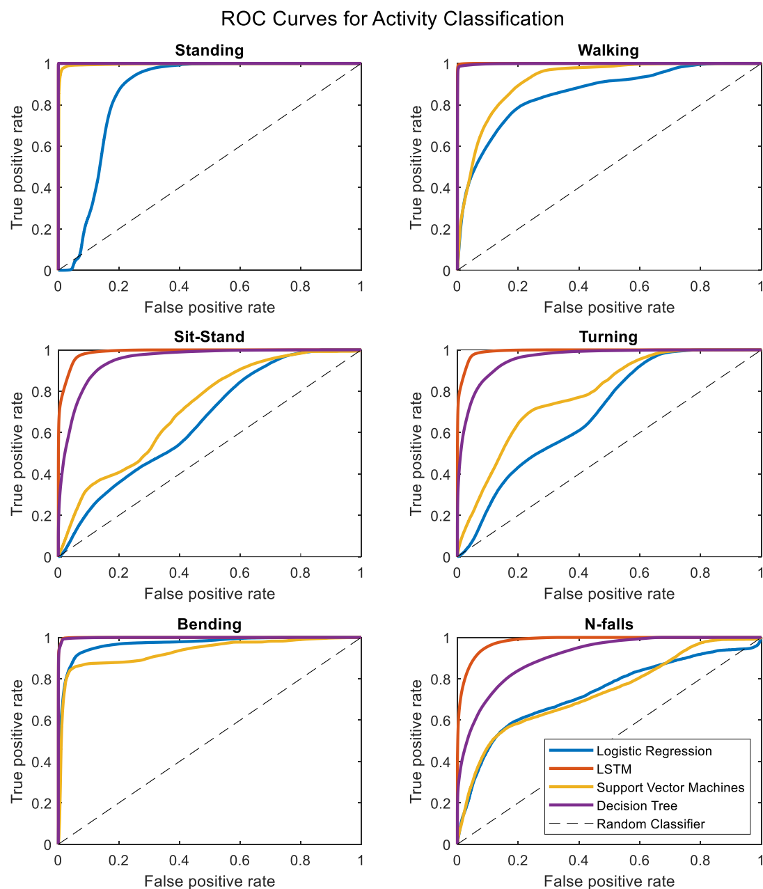
Fig 4. Receiver operating characteristic curves for four binary classifiers plotted separately for each activity.
