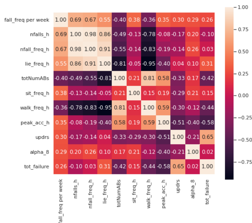
Fig 5. Correlation matrix including the first 10 features with the most correlation with the fall frequency of patients at home.
