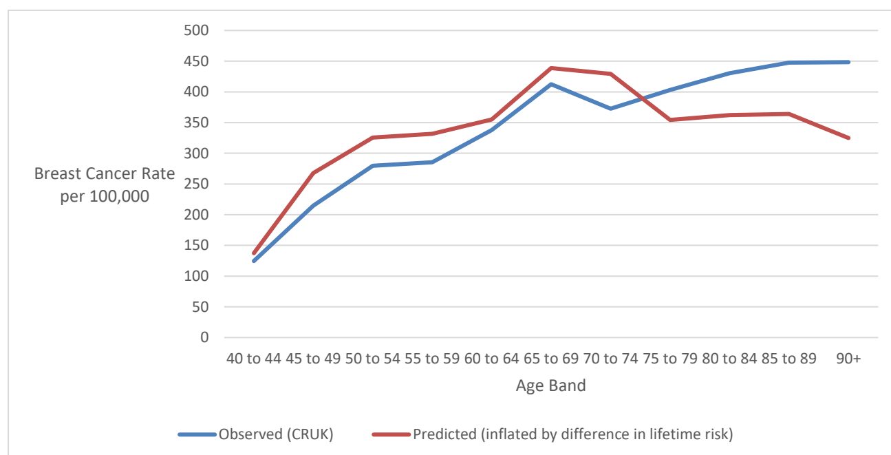
Figure 2: Inflation of predicted incidence rates estimated by MANC-RISK-SCREEN by the proportional difference in lifetime risk
