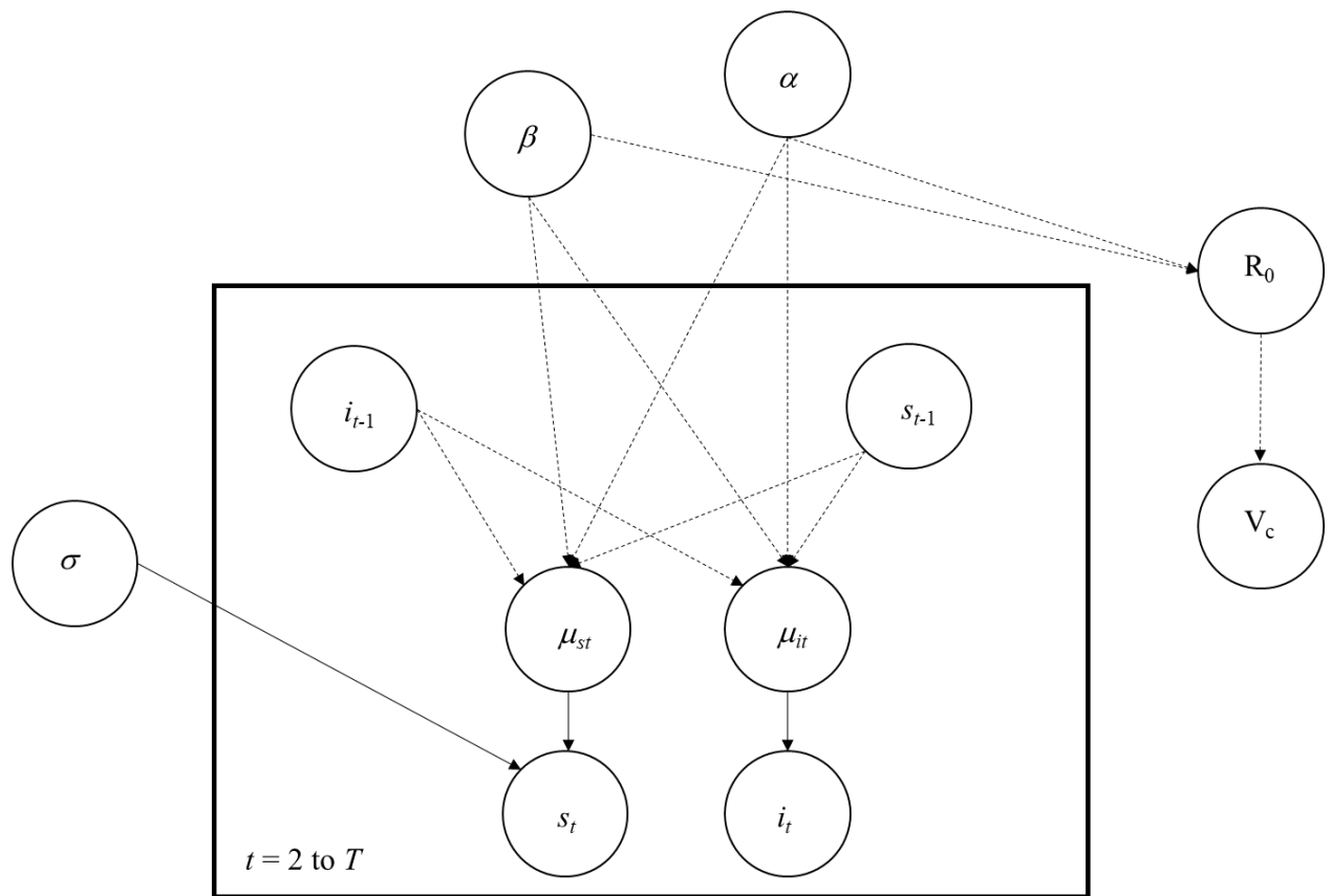
Figure 1 The directed acyclic graph model for estimating the spread of human moneypox
