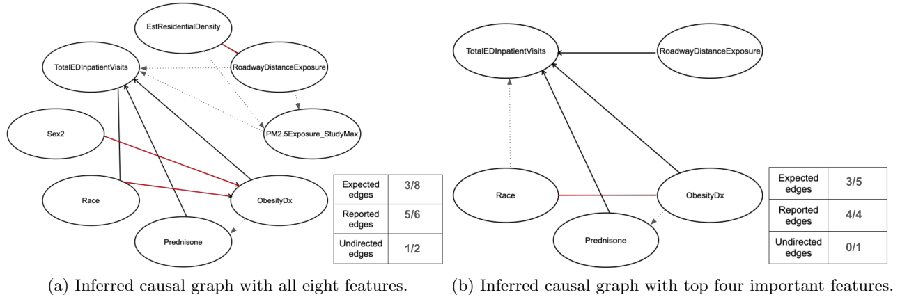
Fig. 3: Inferred causal graph. Solid black lines represent true positives, dashed lines represent false negatives and red lines represents false positives
