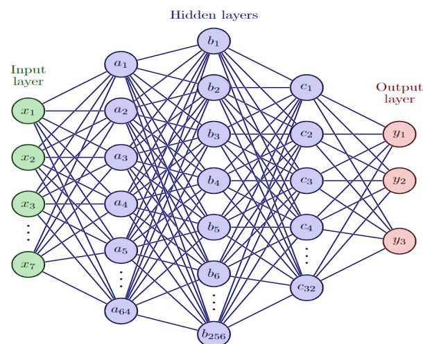
Figure 4. Architecture of Clinical Factors Neural Network
