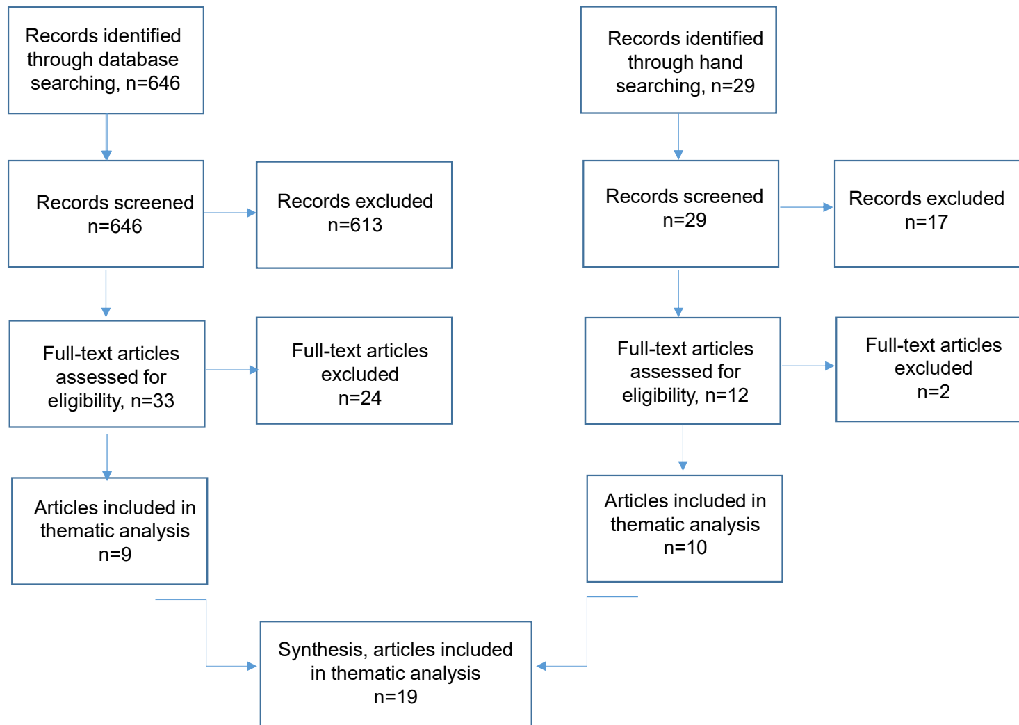
Appendix Figure 1. Flow chart scoping review
