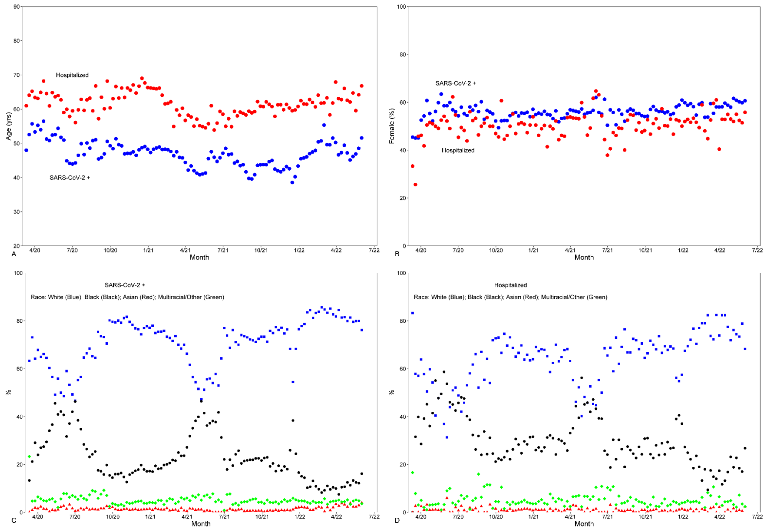
Figure 2: Trends in demographics. Symbols are 1-week averages. In panels A and B, blue symbols refer to persons testing positive for SARS-CoV-2 (SARS-CoV-2 +), and red symbols refer to patients admitted with COVID-19. A) Mean age. B)
