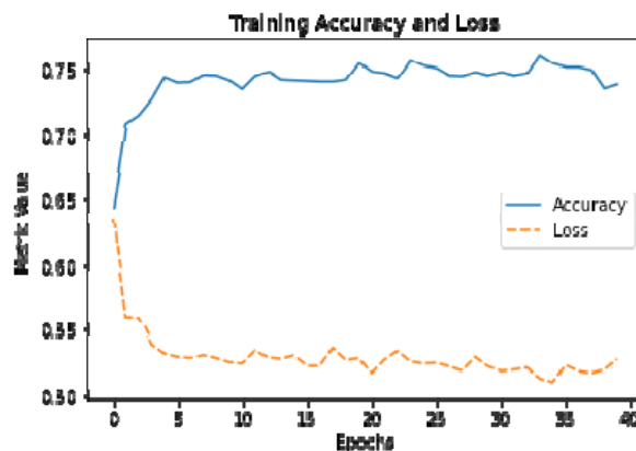
Figure 2. Training accuracy and loss curve
